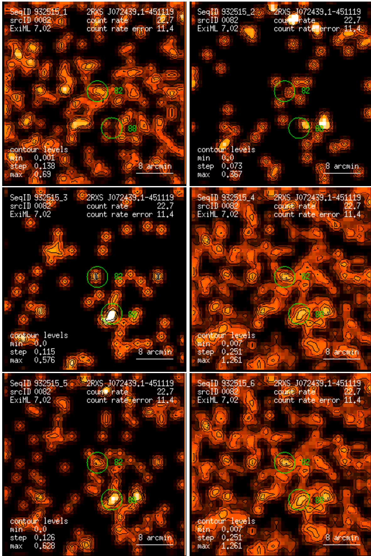
Figure 82: RASS 932515: detection 0082: band rate images, Gaussian filter: (1) PSPC channels 11 – 41, (2) 52 – 90, (3) 91 – 201, (4) 11 – 235, (5) 52 – 201, (6) 11 – 201. Broad band rates in counts/ks. Band rate contour levels in counts/ks/arcmin 2 .
