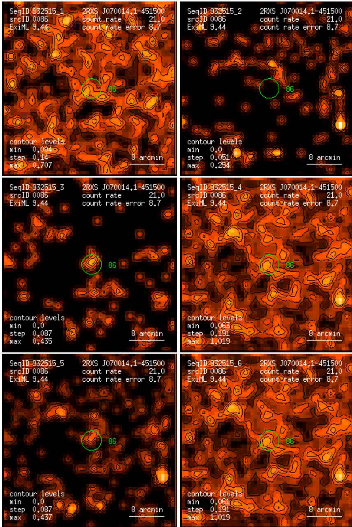
Figure 86: RASS 932515: detection 0086: band rate images, Gaussian filter: (1) PSPC channels 11 – 41, (2) 52 – 90, (3) 91 – 201, (4) 11 – 235, (5) 52 – 201, (6) 11 – 201. Broad band rates in counts/ks. Band rate contour levels in counts/ks/arcmin 2 .
