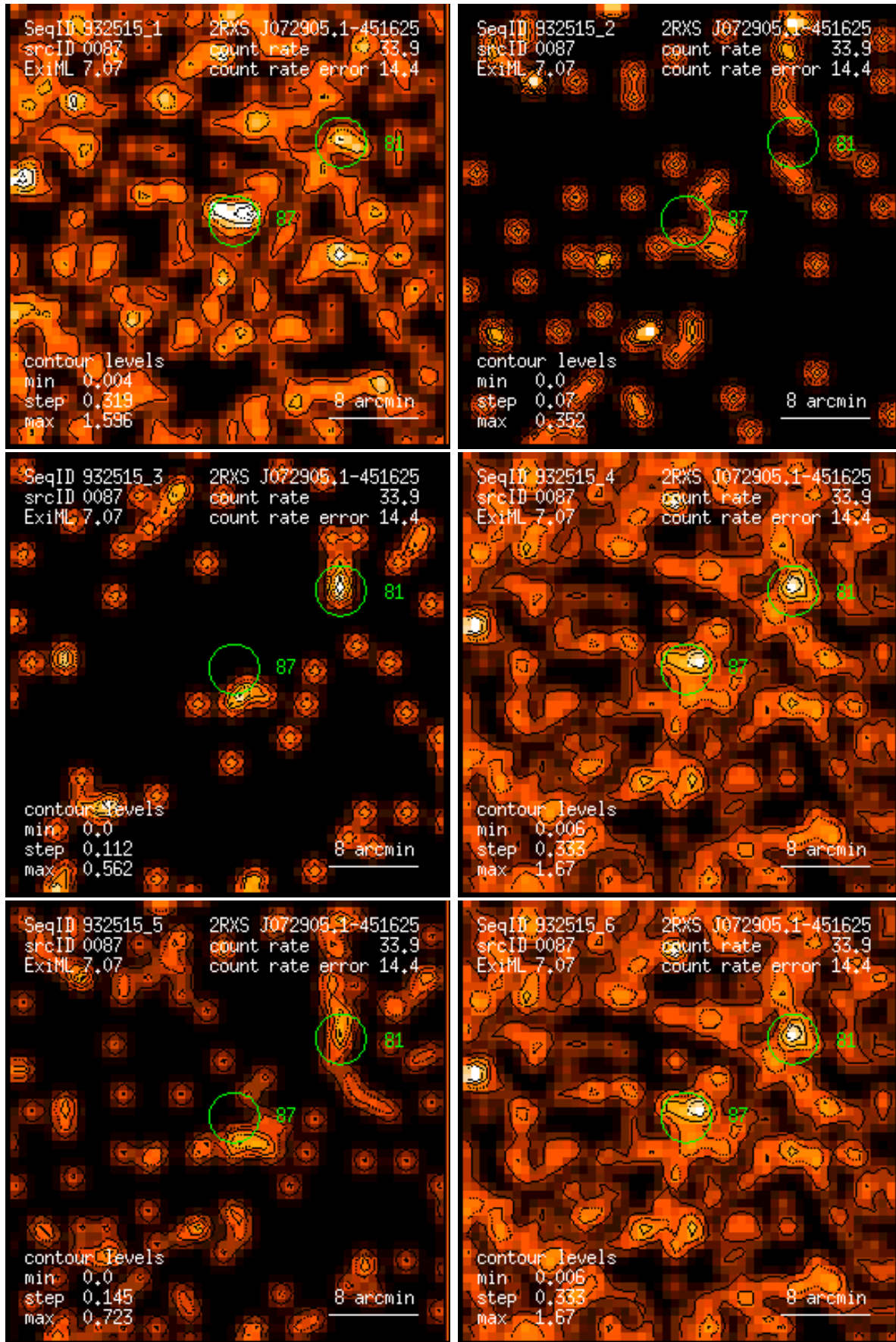
Figure 87: RASS 932515: detection 0087: band rate images, Gaussian filter: (1) PSPC channels 11 – 41, (2) 52 – 90, (3) 91 – 201, (4) 11 – 235, (5) 52 – 201, (6) 11 – 201. Broad band rates in counts/ks. Band rate contour levels in counts/ks/arcmin 2 .
