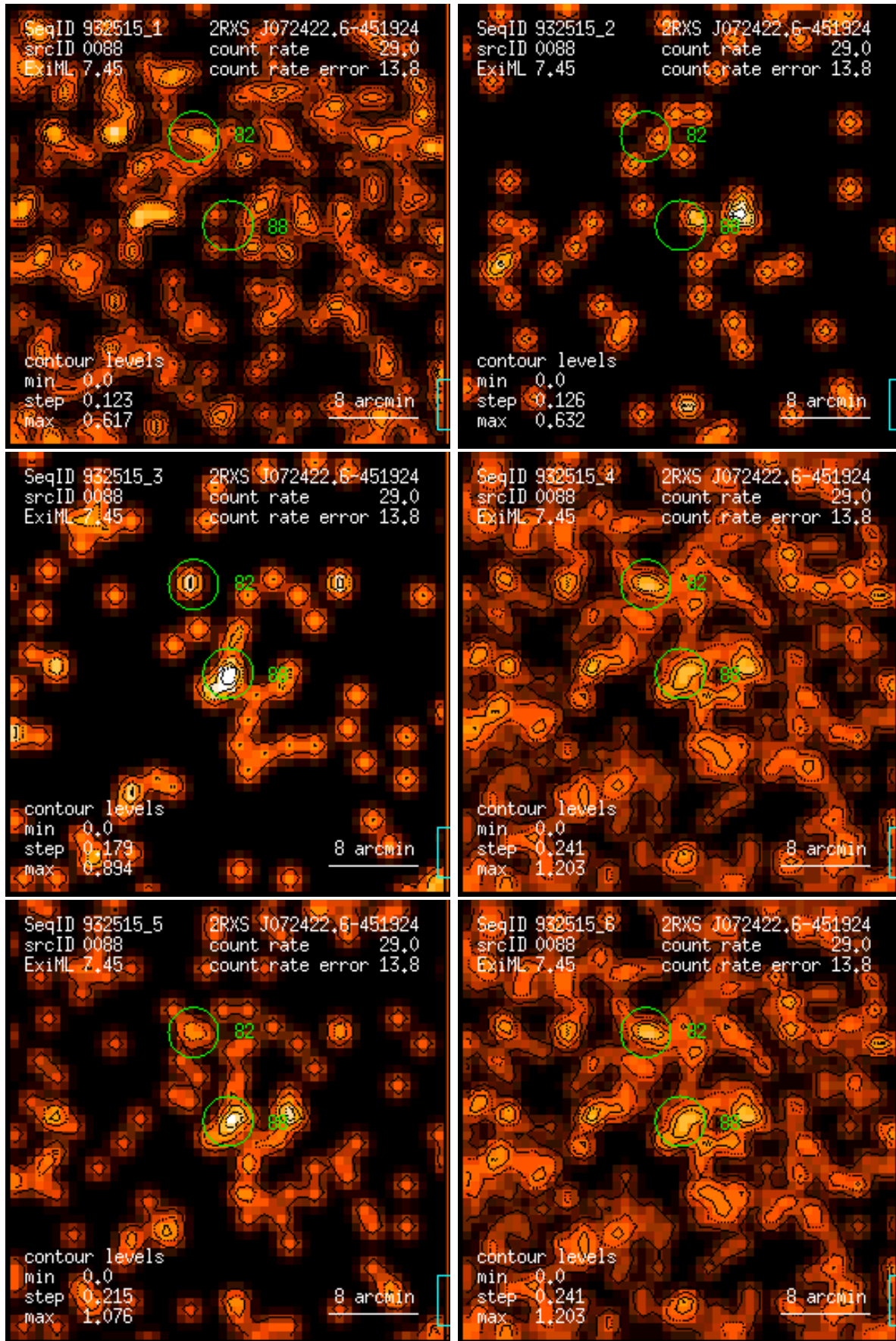
Figure 88: RASS 932515: detection 0088: band rate images, Gaussian filter: (1) PSPC channels 11 – 41, (2) 52 – 90, (3) 91 – 201, (4) 11 – 235, (5) 52 – 201, (6) 11 – 201. Broad band rates in counts/ks. Band rate contour levels in counts/ks/arcmin 2 .
