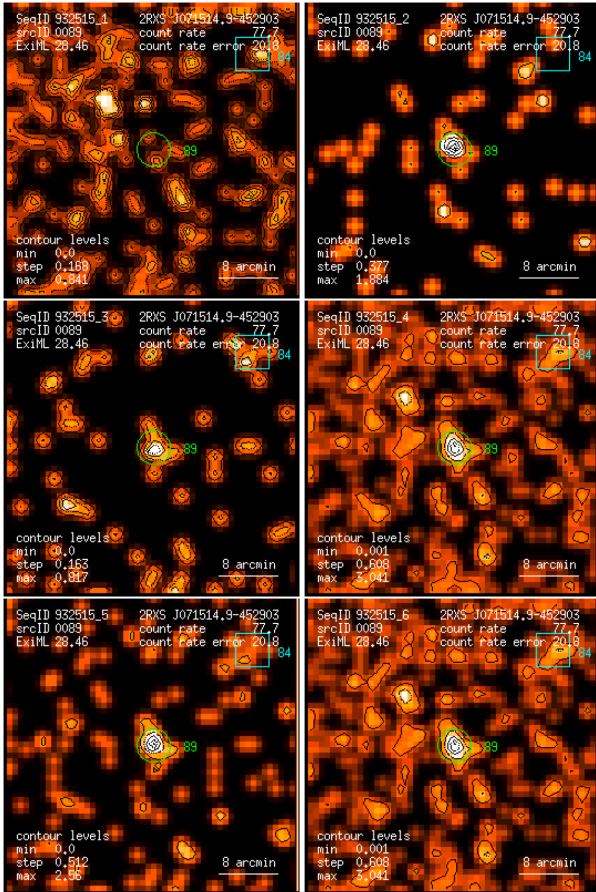
Figure 89: RASS 932515: detection 0089: band rate images, Gaussian filter: (1) PSPC channels 11 – 41, (2) 52 – 90, (3) 91 – 201, (4) 11 – 235, (5) 52 – 201, (6) 11 – 201. Broad band rates in counts/ks. Band rate contour levels in counts/ks/arcmin 2 .
