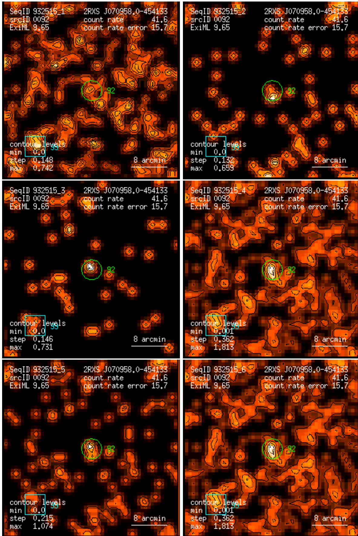
Figure 92: RASS 932515: detection 0092: band rate images, Gaussian filter: (1) PSPC channels 11 – 41, (2) 52 – 90, (3) 91 – 201, (4) 11 – 235, (5) 52 – 201, (6) 11 – 201. Broad band rates in counts/ks. Band rate contour levels in counts/ks/arcmin 2 .
