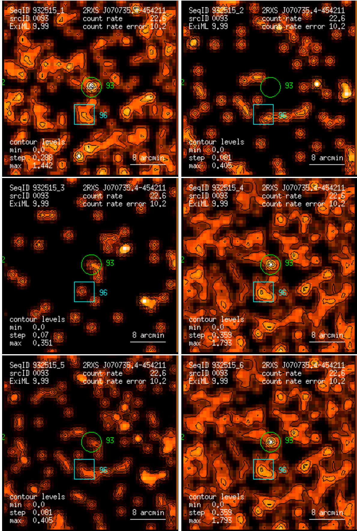
Figure 93: RASS 932515: detection 0093: band rate images, Gaussian filter: (1) PSPC channels 11 – 41, (2) 52 – 90, (3) 91 – 201, (4) 11 – 235, (5) 52 – 201, (6) 11 – 201. Broad band rates in counts/ks. Band rate contour levels in counts/ks/arcmin 2 .
