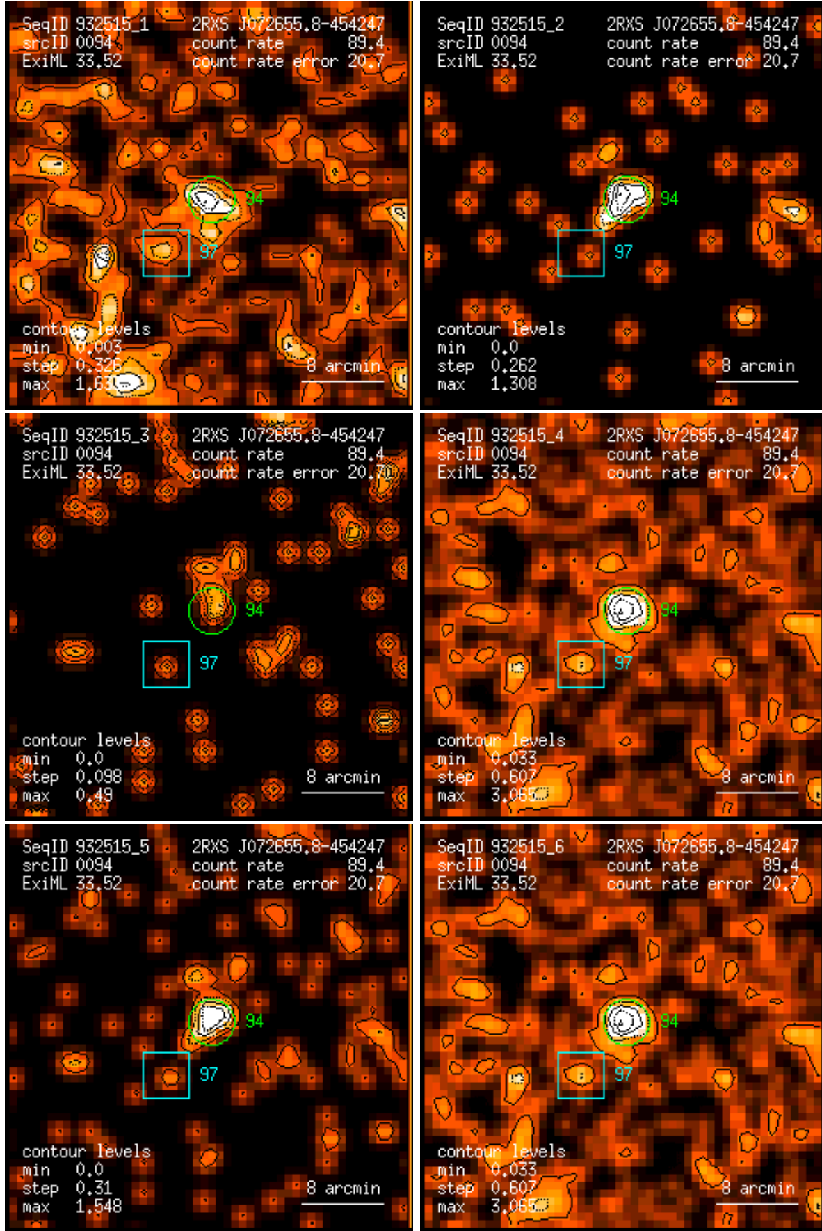
Figure 94: RASS 932515: detection 0094: band rate images, Gaussian filter: (1) PSPC channels 11 – 41, (2) 52 – 90, (3) 91 – 201, (4) 11 – 235, (5) 52 – 201, (6) 11 – 201. Broad band rates in counts/ks. Band rate contour levels in counts/ks/arcmin 2 .
