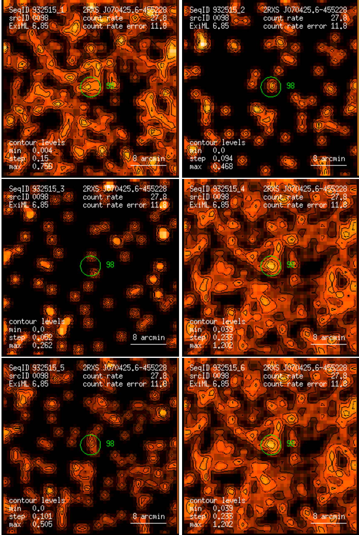
Figure 98: RASS 932515: detection 0098: band rate images, Gaussian filter: (1) PSPC channels 11 – 41, (2) 52 – 90, (3) 91 – 201, (4) 11 – 235, (5) 52 – 201, (6) 11 – 201. Broad band rates in counts/ks. Band rate contour levels in counts/ks/arcmin 2 .
