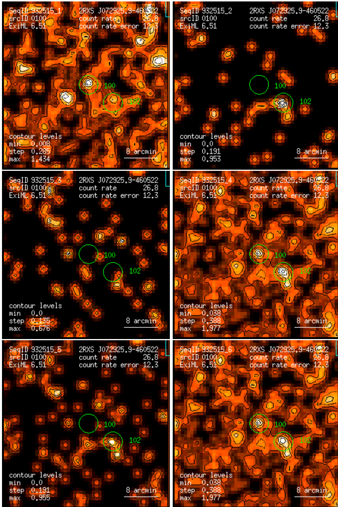
Figure 100: RASS 932515: detection 0100: band rate images, Gaussian filter: (1) PSPC channels 11 – 41, (2) 52 – 90, (3) 91 – 201, (4) 11 – 235, (5) 52 – 201, (6) 11 – 201. Broad band rates in counts/ks. Band rate contour levels in counts/ks/arcmin 2 .
