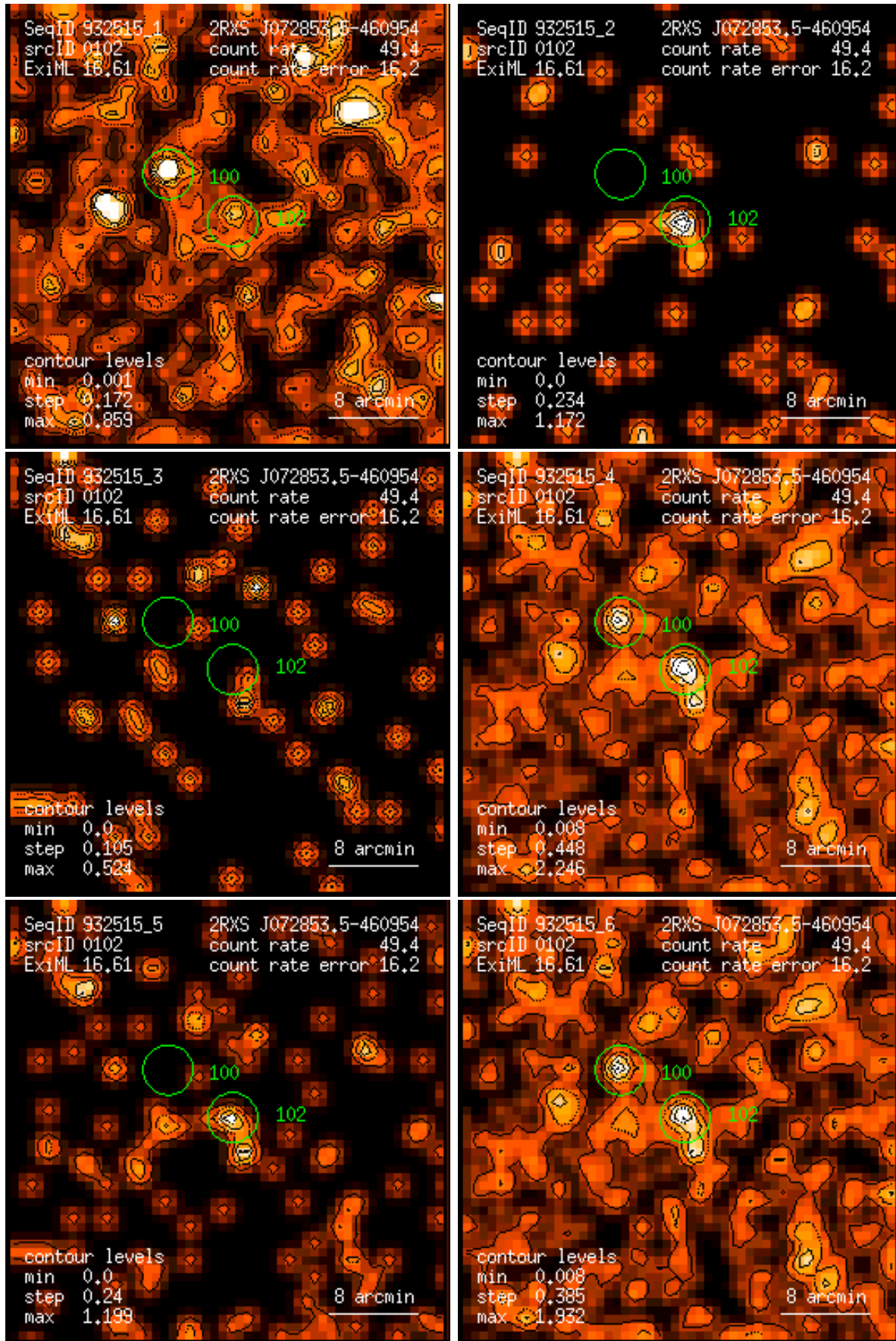
Figure 102: RASS 932515: detection 0102: band rate images, Gaussian filter: (1) PSPC channels 11 – 41, (2) 52 – 90, (3) 91 – 201, (4) 11 – 235, (5) 52 – 201, (6) 11 – 201. Broad band rates in counts/ks. Band rate contour levels in counts/ks/arcmin 2 .
