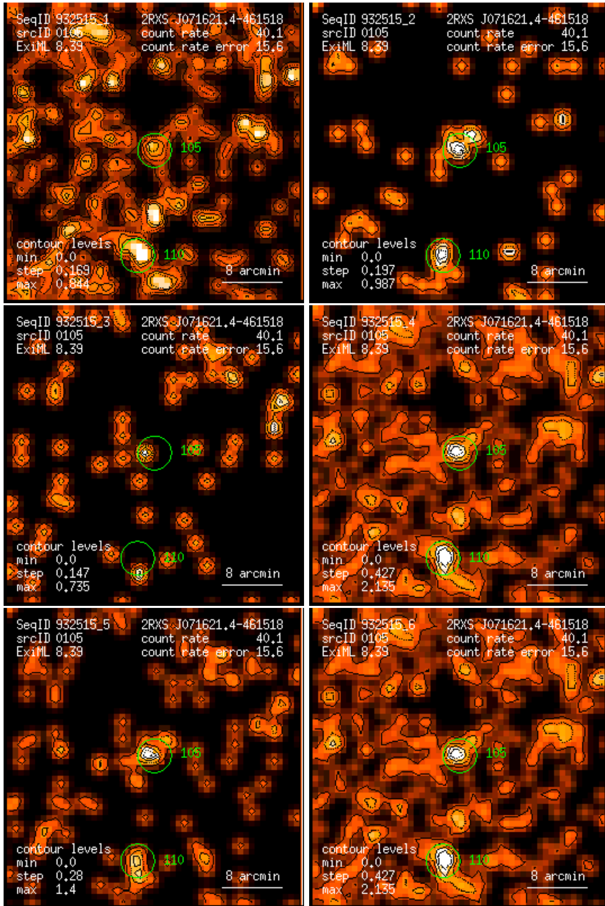
Figure 105: RASS 932515: detection 0105: band rate images, Gaussian filter: (1) PSPC channels 11 – 41, (2) 52 – 90, (3) 91 – 201, (4) 11 – 235, (5) 52 – 201, (6) 11 – 201. Broad band rates in counts/ks. Band rate contour levels in counts/ks/arcmin 2 .
