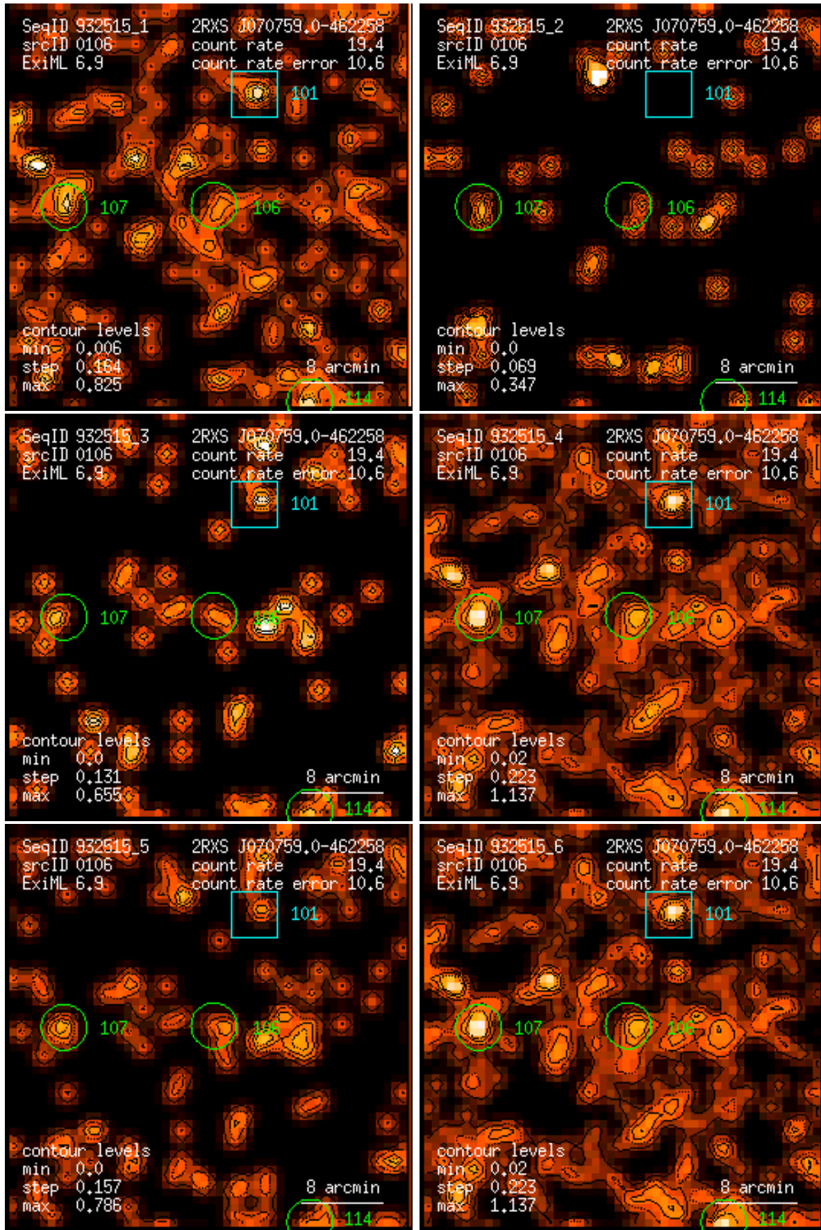
Figure 106: RASS 932515: detection 0106: band rate images, Gaussian filter: (1) PSPC channels 11 – 41, (2) 52 – 90, (3) 91 – 201, (4) 11 – 235, (5) 52 – 201, (6) 11 – 201. Broad band rates in counts/ks. Band rate contour levels in counts/ks/arcmin 2 .
