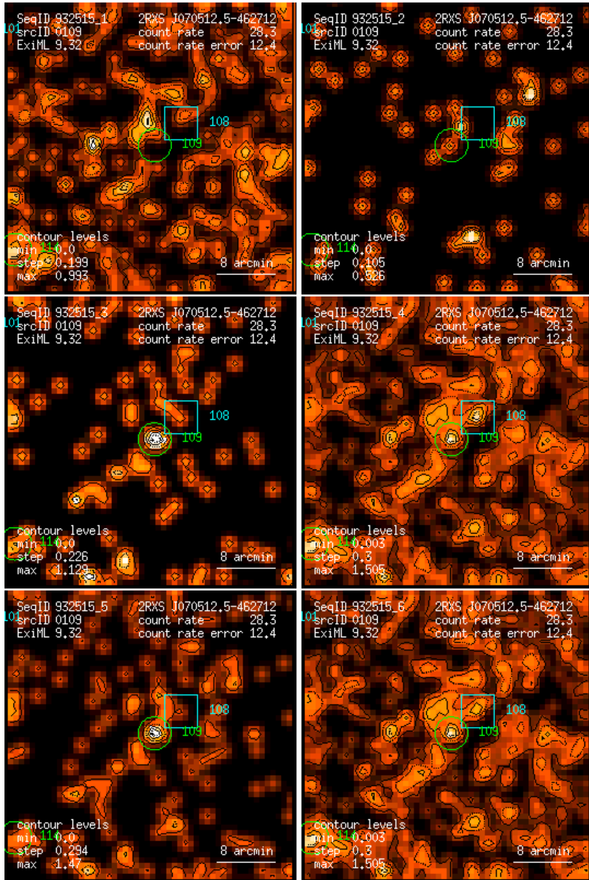
Figure 109: RASS 932515: detection 0109: band rate images, Gaussian filter: (1) PSPC channels 11 – 41, (2) 52 – 90, (3) 91 – 201, (4) 11 – 235, (5) 52 – 201, (6) 11 – 201. Broad band rates in counts/ks. Band rate contour levels in counts/ks/arcmin 2 .
