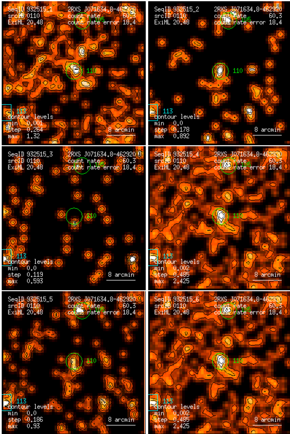
Figure 110: RASS 932515: detection 0110: band rate images, Gaussian filter: (1) PSPC channels 11 – 41, (2) 52 – 90, (3) 91 – 201, (4) 11 – 235, (5) 52 – 201, (6) 11 – 201. Broad band rates in counts/ks. Band rate contour levels in counts/ks/arcmin 2 .
