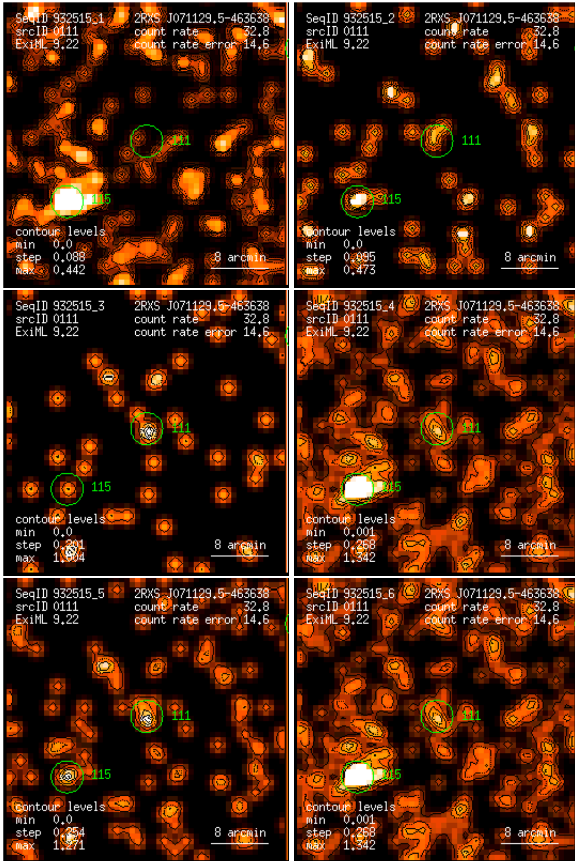
Figure 111: RASS 932515: detection 0111: band rate images, Gaussian filter: (1) PSPC channels 11 – 41, (2) 52 – 90, (3) 91 – 201, (4) 11 – 235, (5) 52 – 201, (6) 11 – 201. Broad band rates in counts/ks. Band rate contour levels in counts/ks/arcmin 2 .
