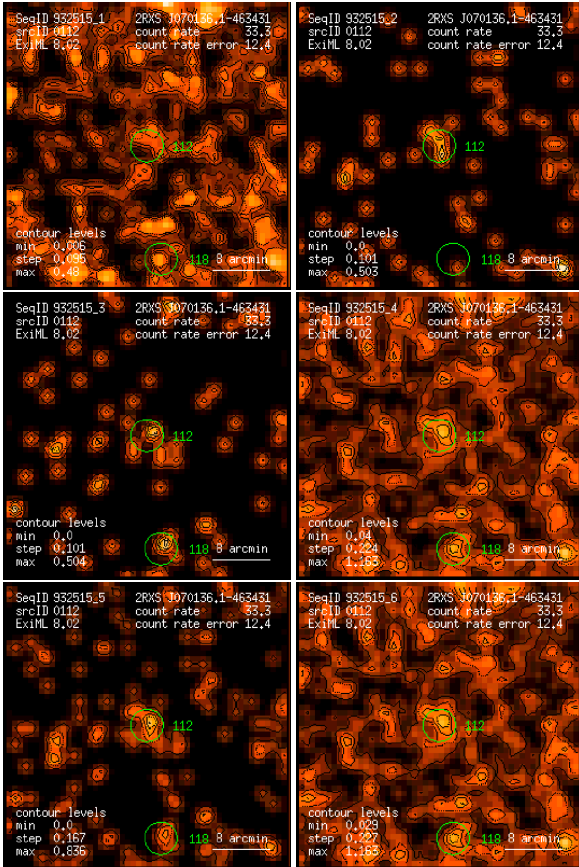
Figure 112: RASS 932515: detection 0112: band rate images, Gaussian filter: (1) PSPC channels 11 – 41, (2) 52 – 90, (3) 91 – 201, (4) 11 – 235, (5) 52 – 201, (6) 11 – 201. Broad band rates in counts/ks. Band rate contour levels in counts/ks/arcmin 2 .
