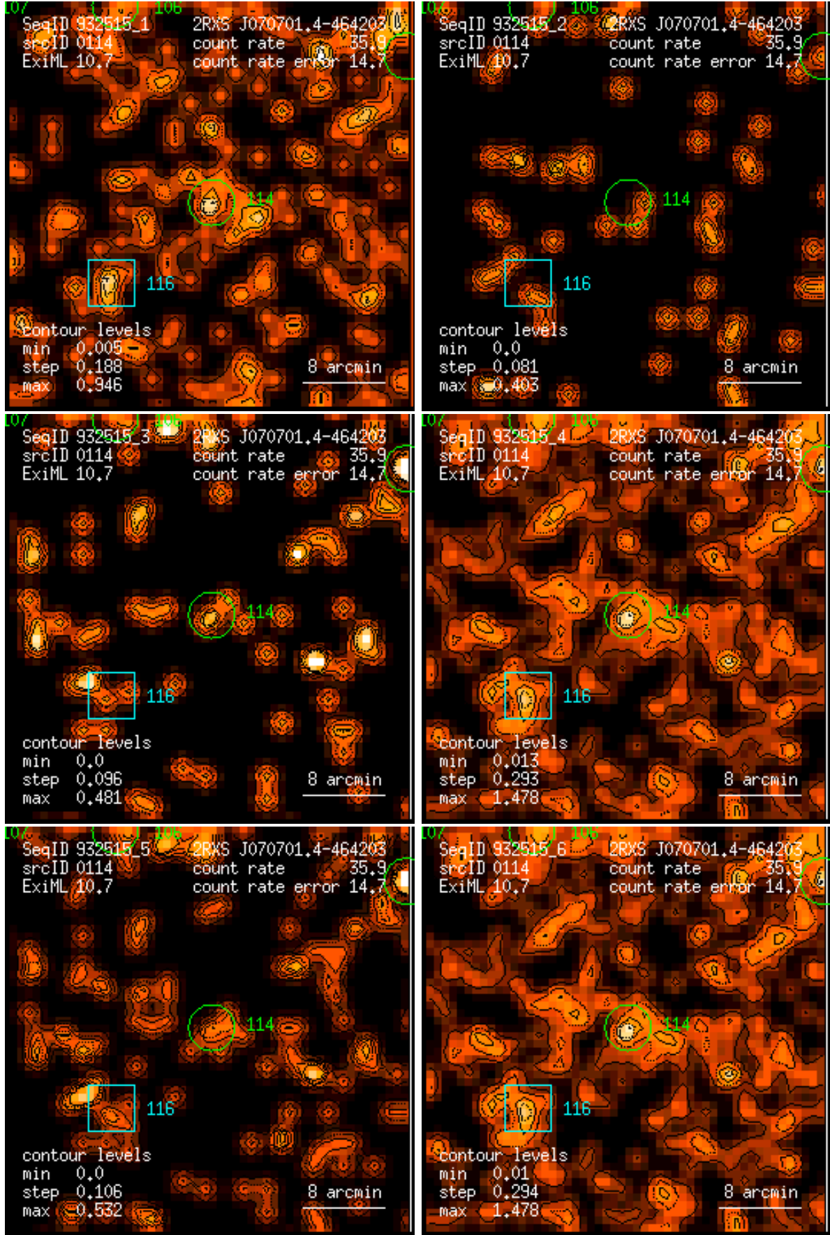
Figure 114: RASS 932515: detection 0114: band rate images, Gaussian filter: (1) PSPC channels 11 – 41, (2) 52 – 90, (3) 91 – 201, (4) 11 – 235, (5) 52 – 201, (6) 11 – 201. Broad band rates in counts/ks. Band rate contour levels in counts/ks/arcmin 2 .
