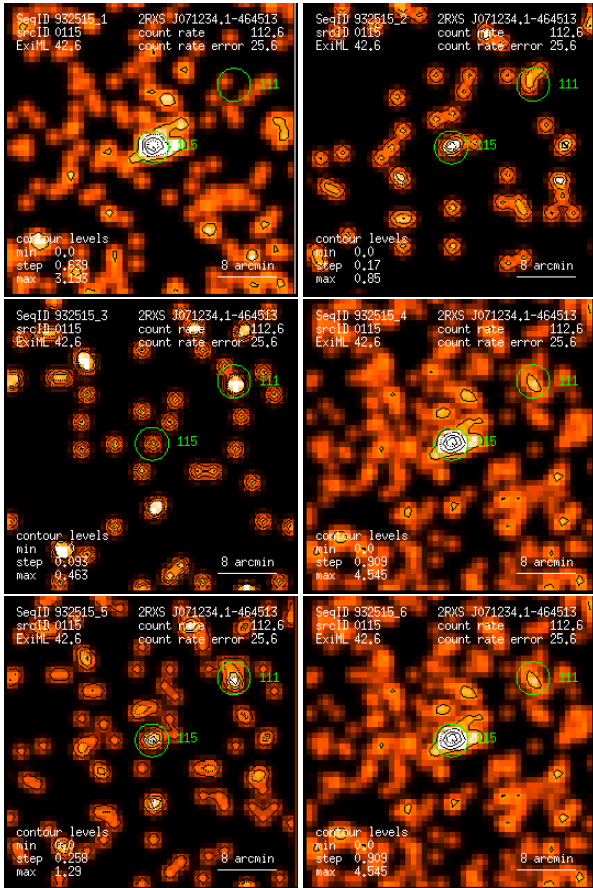
Figure 115: RASS 932515: detection 0115: band rate images, Gaussian filter: (1) PSPC channels 11 – 41, (2) 52 – 90, (3) 91 – 201, (4) 11 – 235, (5) 52 – 201, (6) 11 – 201. Broad band rates in counts/ks. Band rate contour levels in counts/ks/arcmin 2 .
