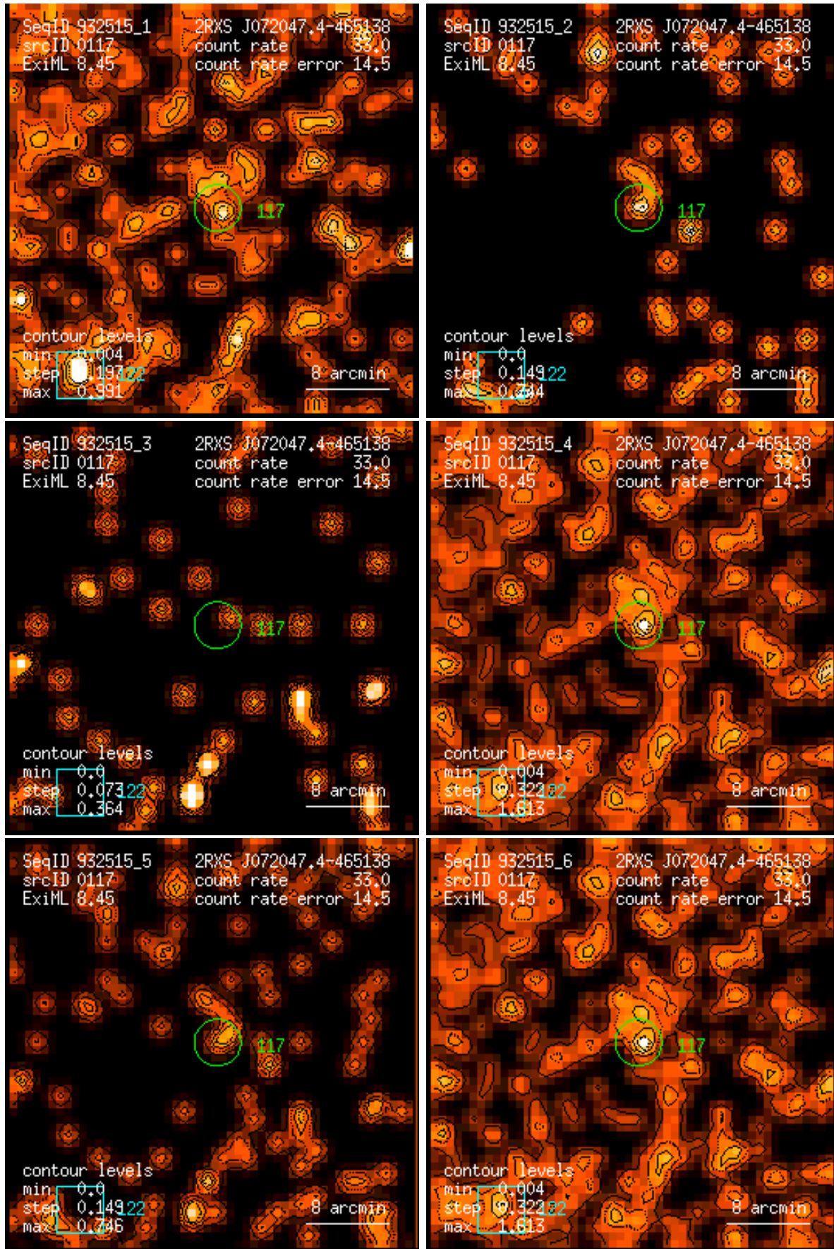
Figure 117: RASS 932515: detection 0117: band rate images, Gaussian filter: (1) PSPC channels 11 – 41, (2) 52 – 90, (3) 91 – 201, (4) 11 – 235, (5) 52 – 201, (6) 11 – 201. Broad band rates in counts/ks. Band rate contour levels in counts/ks/arcmin 2 .
