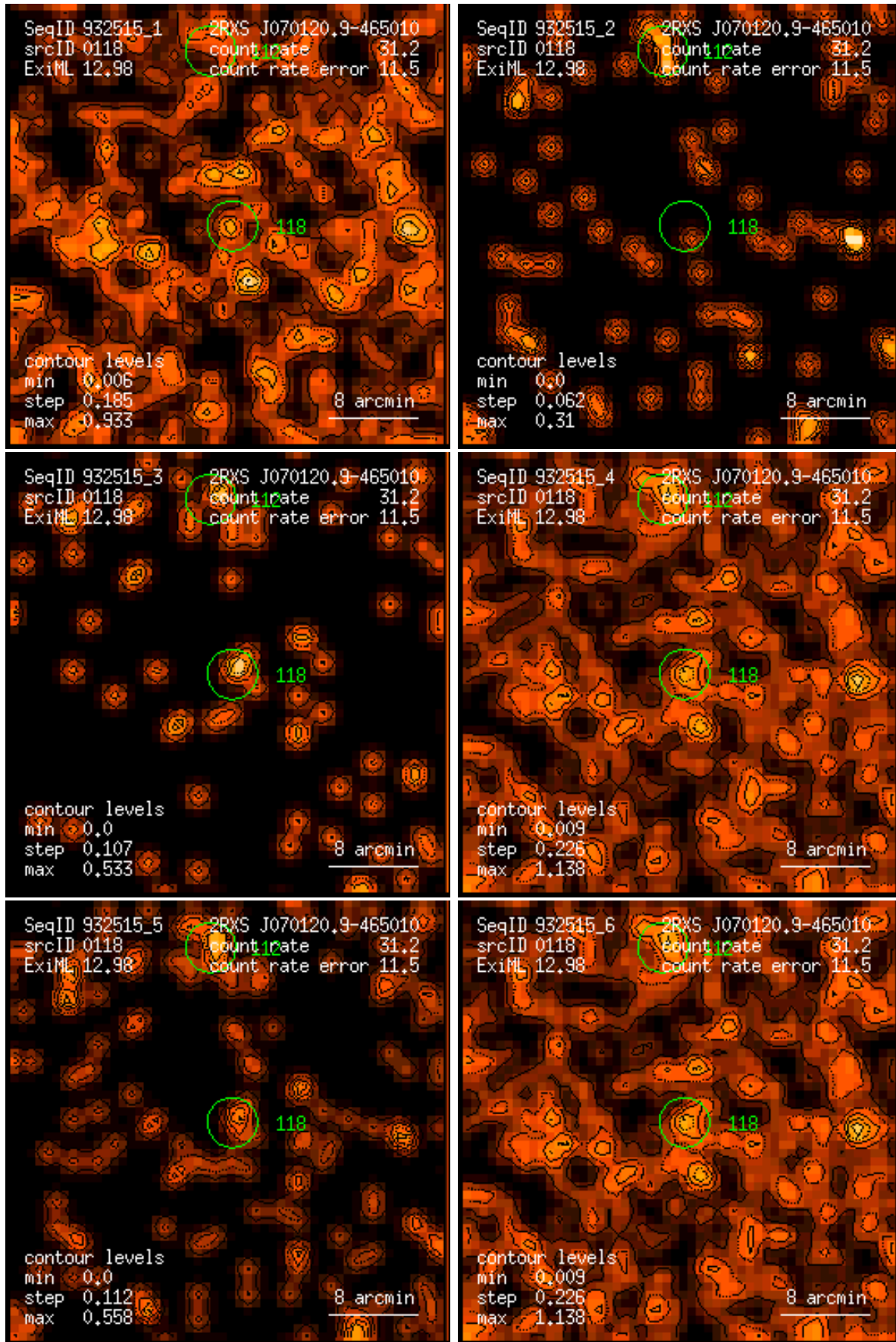
Figure 118: RASS 932515: detection 0118: band rate images, Gaussian filter: (1) PSPC channels 11 – 41, (2) 52 – 90, (3) 91 – 201, (4) 11 – 235, (5) 52 – 201, (6) 11 – 201. Broad band rates in counts/ks. Band rate contour levels in counts/ks/arcmin 2 .
