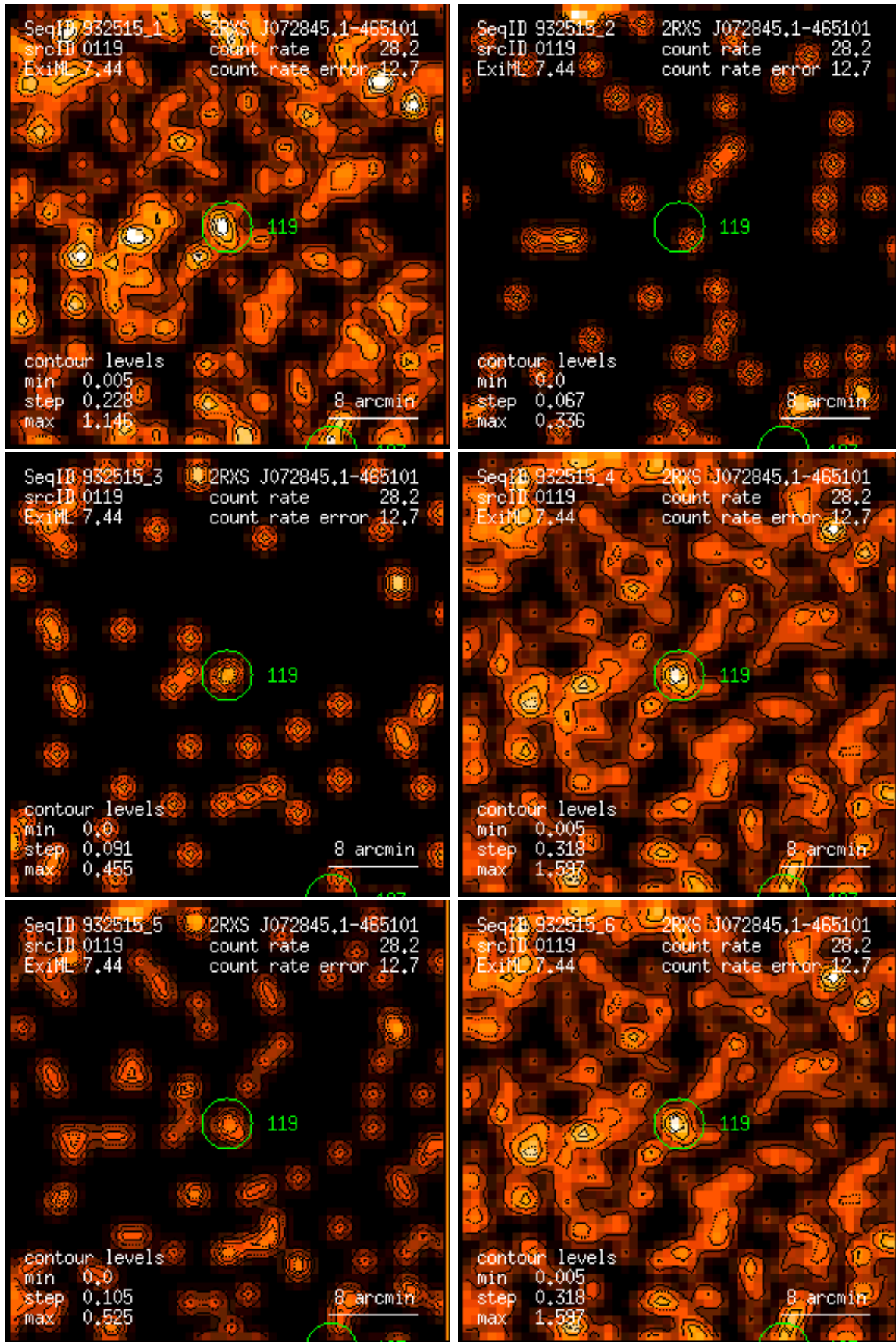
Figure 119: RASS 932515: detection 0119: band rate images, Gaussian filter: (1) PSPC channels 11 – 41, (2) 52 – 90, (3) 91 – 201, (4) 11 – 235, (5) 52 – 201, (6) 11 – 201. Broad band rates in counts/ks. Band rate contour levels in counts/ks/arcmin 2 .
