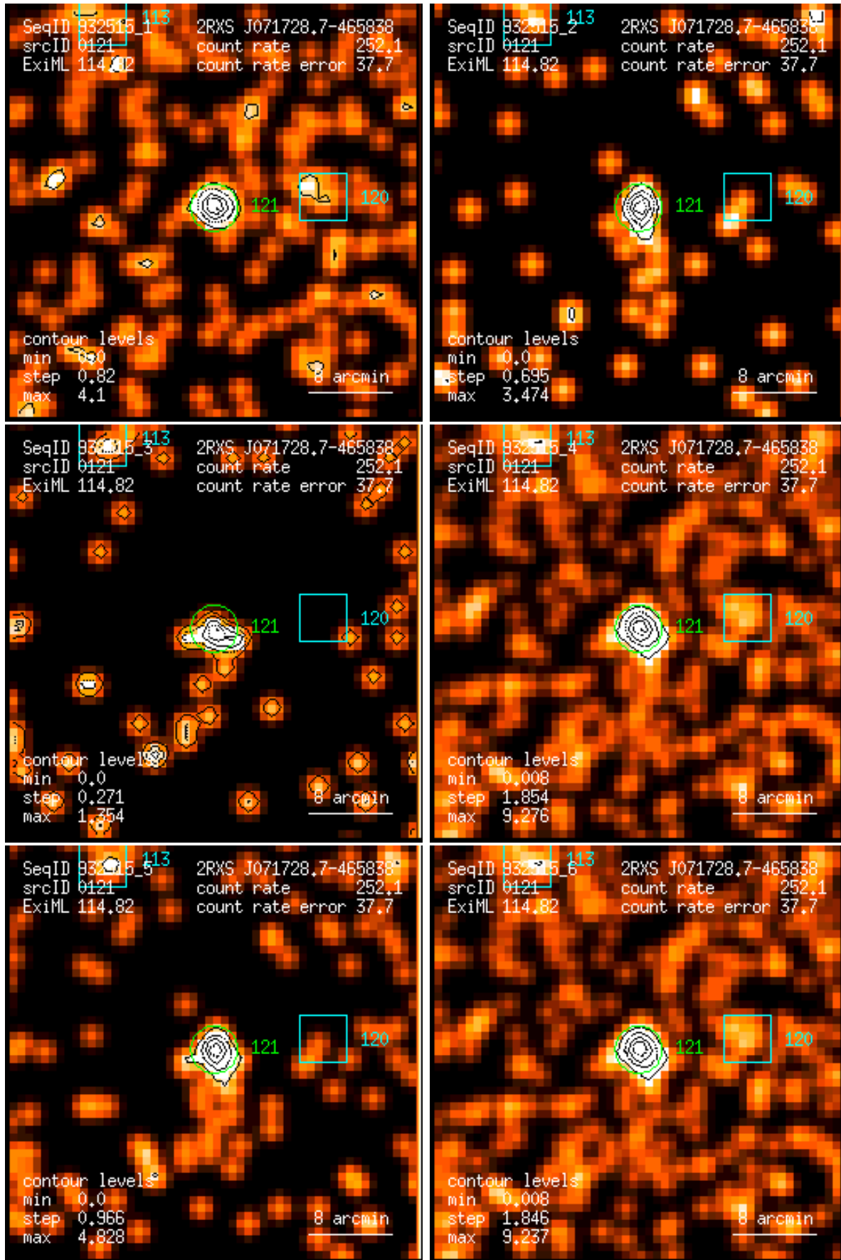
Figure 121: RASS 932515: detection 0121: band rate images, Gaussian filter: (1) PSPC channels 11 – 41, (2) 52 – 90, (3) 91 – 201, (4) 11 – 235, (5) 52 – 201, (6) 11 – 201. Broad band rates in counts/ks. Band rate contour levels in counts/ks/arcmin 2 .
