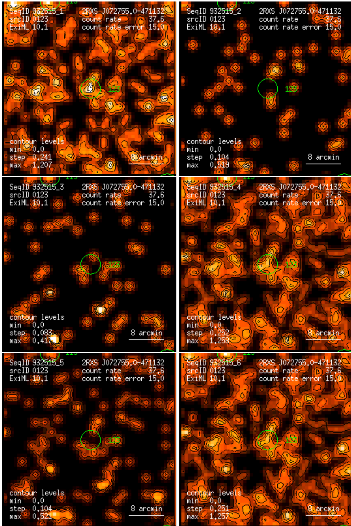
Figure 123: RASS 932515: detection 0123: band rate images, Gaussian filter: (1) PSPC channels 11 – 41, (2) 52 – 90, (3) 91 – 201, (4) 11 – 235, (5) 52 – 201, (6) 11 – 201. Broad band rates in counts/ks. Band rate contour levels in counts/ks/arcmin 2 .
