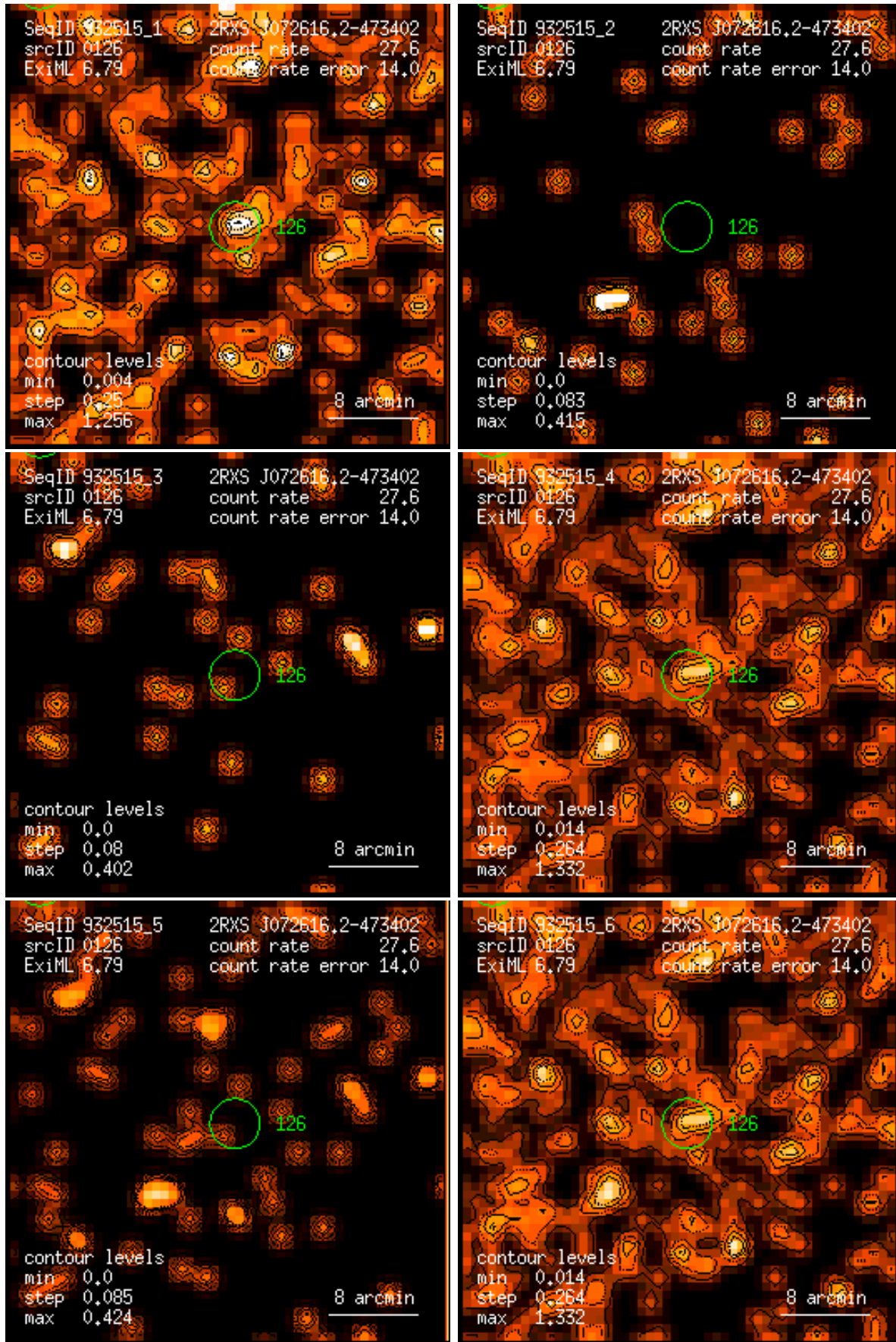
Figure 126: RASS 932515: detection 0126: band rate images, Gaussian filter: (1) PSPC channels 11 – 41, (2) 52 – 90, (3) 91 – 201, (4) 11 – 235, (5) 52 – 201, (6) 11 – 201. Broad band rates in counts/ks. Band rate contour levels in counts/ks/arcmin 2 .
