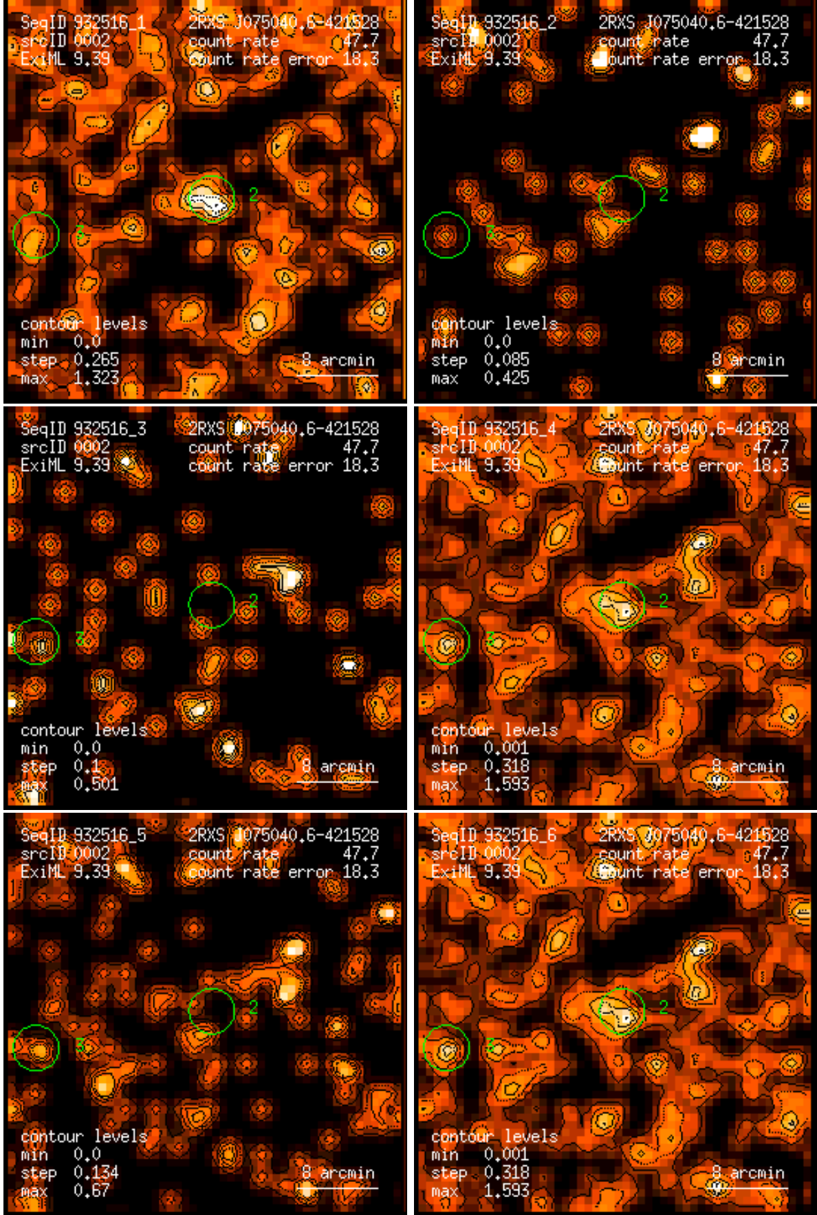
Figure 2: RASS 932516: detection 0002: band rate images, Gaussian filter: (1) PSPC channels 11 – 41, (2) 52 – 90, (3) 91 – 201, (4) 11 – 235, (5) 52 – 201, (6) 11 – 201. Broad band rates in counts/ks. Band rate contour levels in counts/ks/arcmin 2 .
