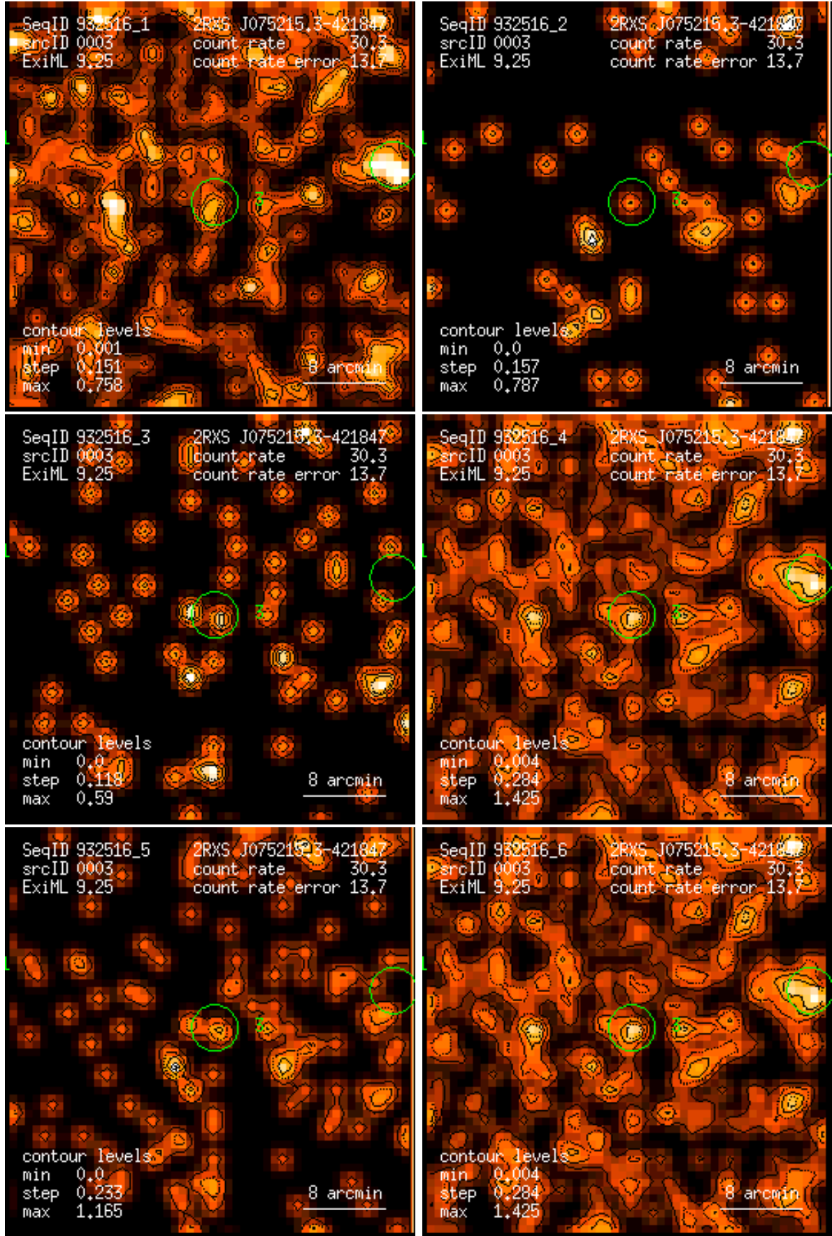
Figure 3: RASS 932516: detection 0003: band rate images, Gaussian filter: (1) PSPC channels 11 – 41, (2) 52 – 90, (3) 91 – 201, (4) 11 – 235, (5) 52 – 201, (6) 11 – 201. Broad band rates in counts/ks. Band rate contour levels in counts/ks/arcmin 2 .
