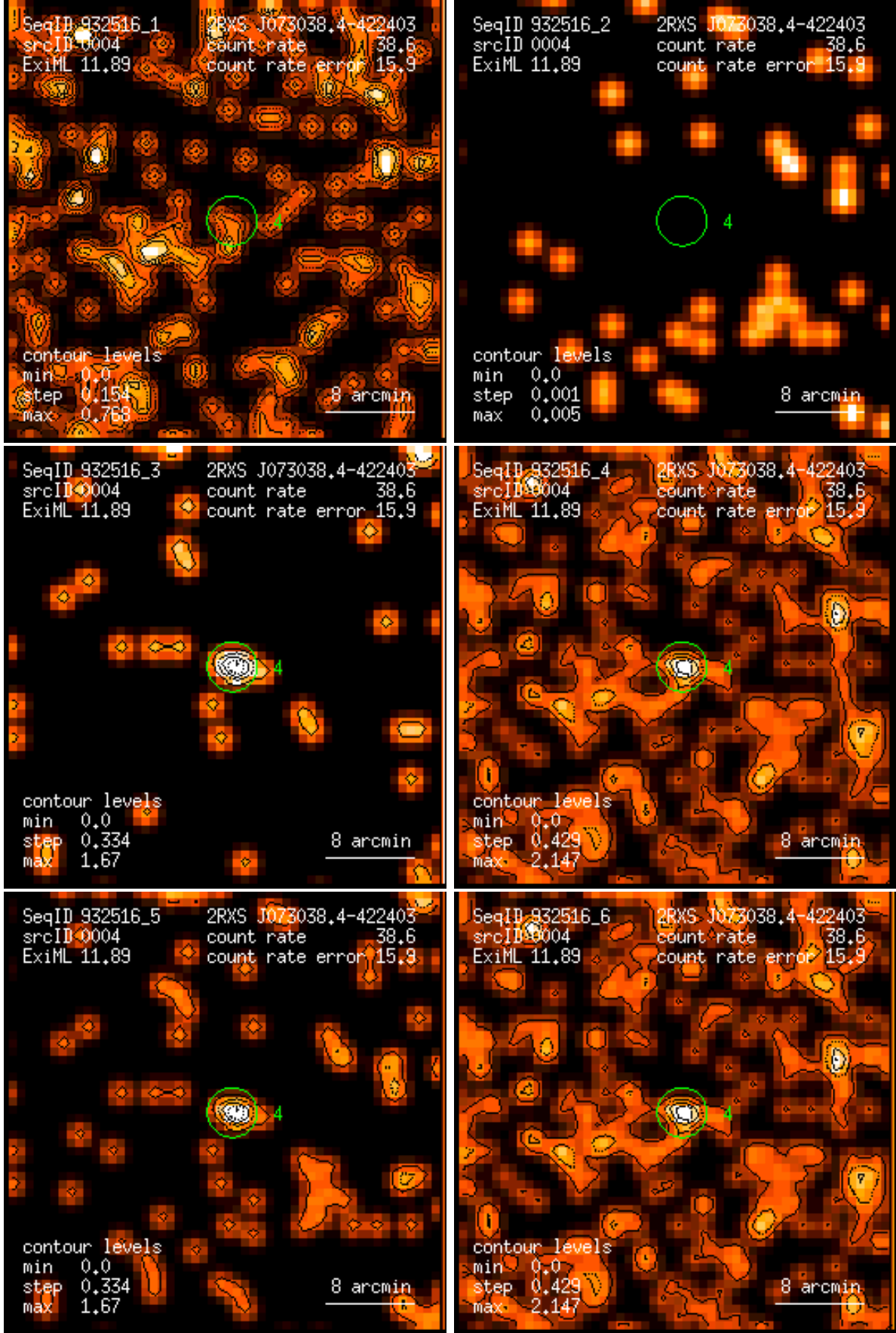
Figure 4: RASS 932516: detection 0004: band rate images, Gaussian filter: (1) PSPC channels 11 – 41, (2) 52 – 90, (3) 91 – 201, (4) 11 – 235, (5) 52 – 201, (6) 11 – 201. Broad band rates in counts/ks. Band rate contour levels in counts/ks/arcmin 2 .
