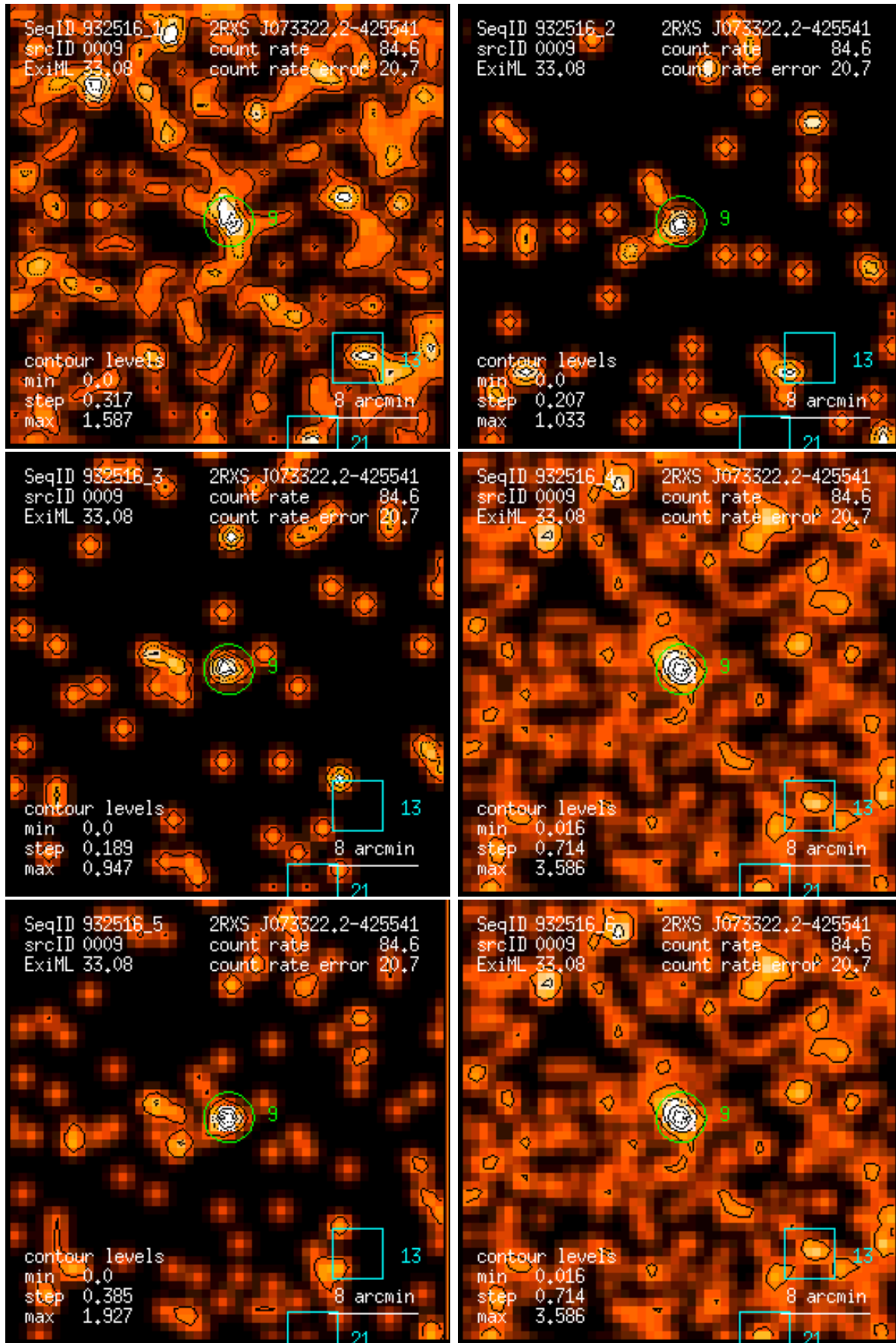
Figure 9: RASS 932516: detection 0009: band rate images, Gaussian filter: (1) PSPC channels 11 – 41, (2) 52 – 90, (3) 91 – 201, (4) 11 – 235, (5) 52 – 201, (6) 11 – 201. Broad band rates in counts/ks. Band rate contour levels in counts/ks/arcmin 2 .
