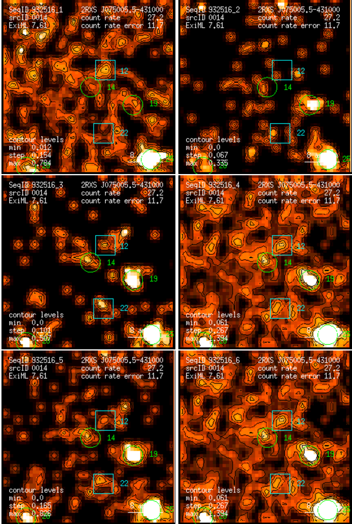
Figure 14: RASS 932516: detection 0014: band rate images, Gaussian filter: (1) PSPC channels 11 – 41, (2) 52 – 90, (3) 91 – 201, (4) 11 – 235, (5) 52 – 201, (6) 11 – 201. Broad band rates in counts/ks. Band rate contour levels in counts/ks/arcmin 2 .
