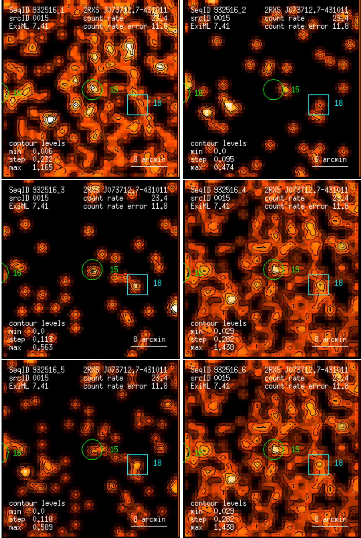
Figure 15: RASS 932516: detection 0015: band rate images, Gaussian filter: (1) PSPC channels 11 – 41, (2) 52 – 90, (3) 91 – 201, (4) 11 – 235, (5) 52 – 201, (6) 11 – 201. Broad band rates in counts/ks. Band rate contour levels in counts/ks/arcmin 2 .
