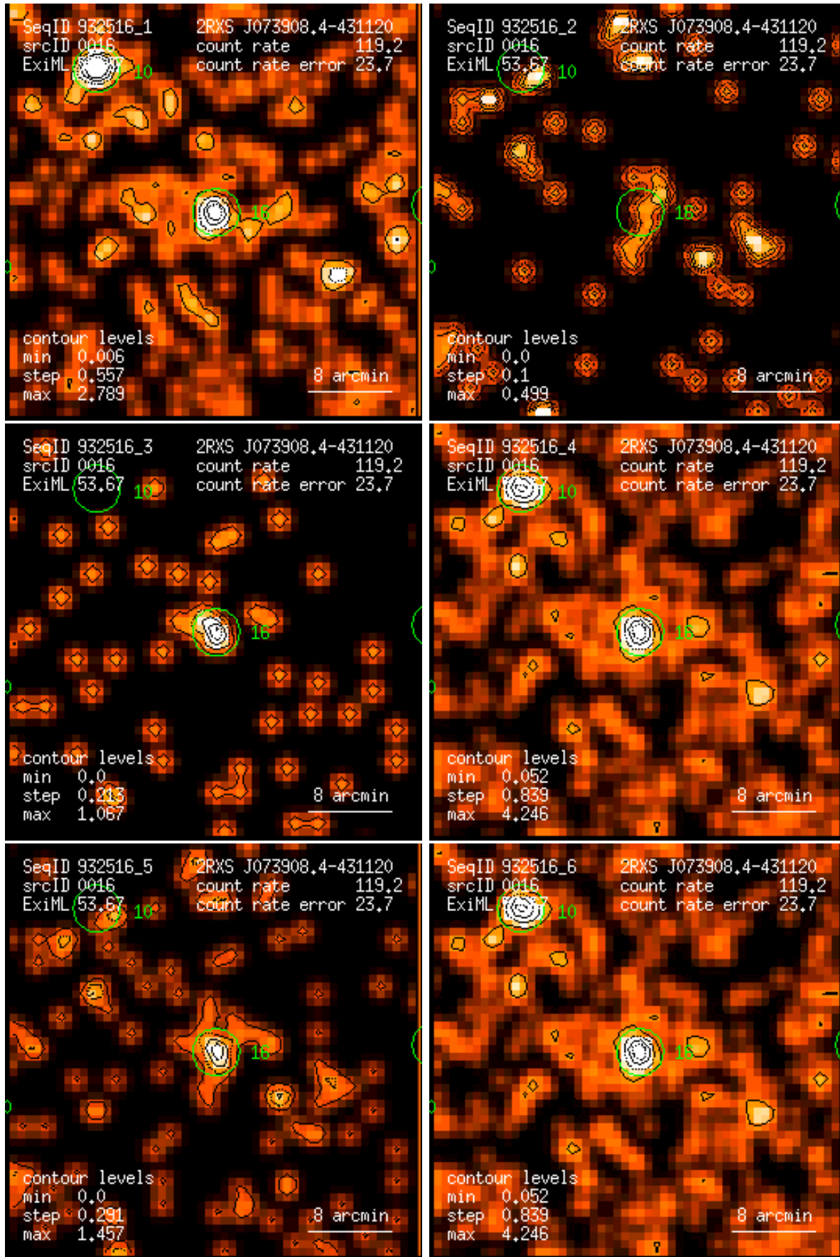
Figure 16: RASS 932516: detection 0016: band rate images, Gaussian filter: (1) PSPC channels 11 – 41, (2) 52 – 90, (3) 91 – 201, (4) 11 – 235, (5) 52 – 201, (6) 11 – 201. Broad band rates in counts/ks. Band rate contour levels in counts/ks/arcmin 2 .
