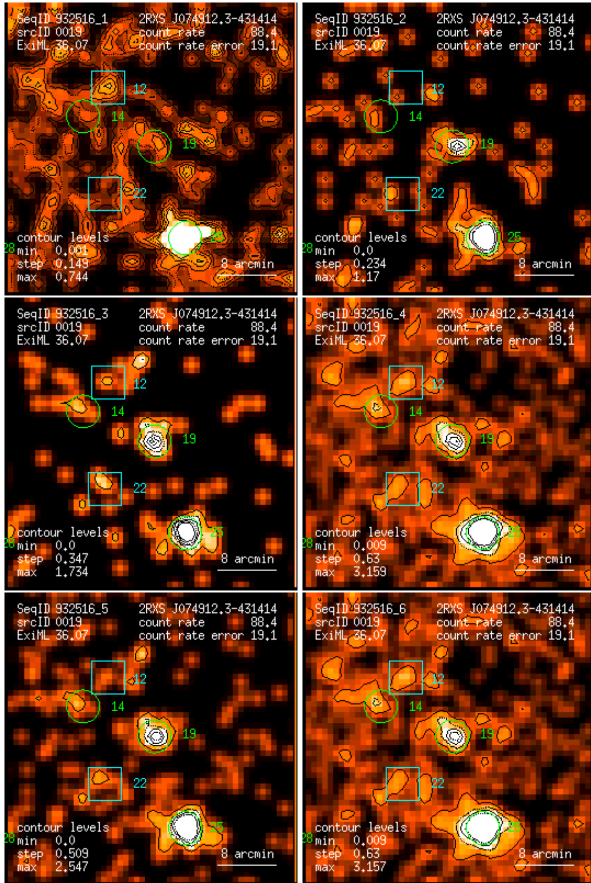
Figure 19: RASS 932516: detection 0019: band rate images, Gaussian filter: (1) PSPC channels 11 – 41, (2) 52 – 90, (3) 91 – 201, (4) 11 – 235, (5) 52 – 201, (6) 11 – 201. Broad band rates in counts/ks. Band rate contour levels in counts/ks/arcmin 2 .
