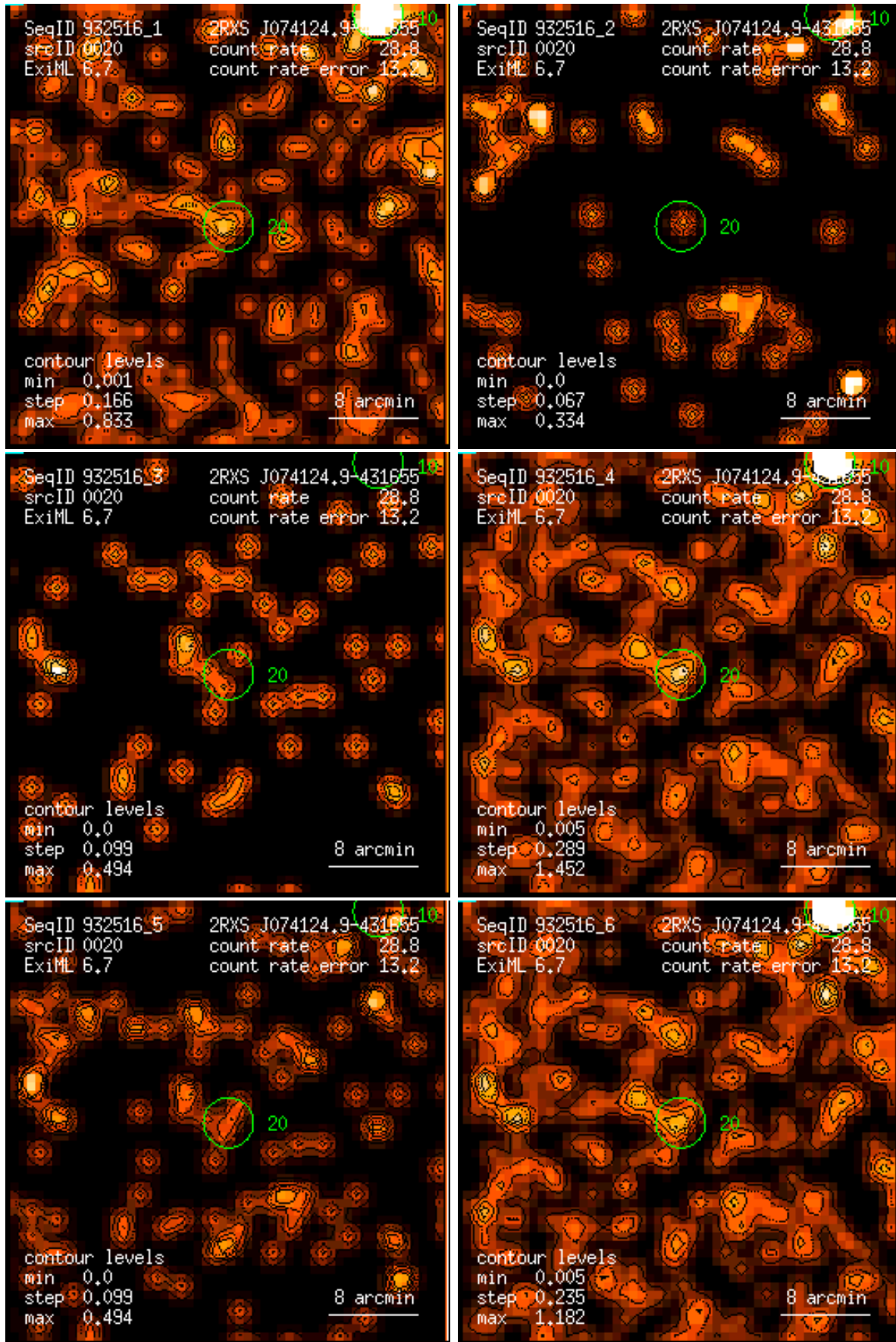
Figure 20: RASS 932516: detection 0020: band rate images, Gaussian filter: (1) PSPC channels 11 – 41, (2) 52 – 90, (3) 91 – 201, (4) 11 – 235, (5) 52 – 201, (6) 11 – 201. Broad band rates in counts/ks. Band rate contour levels in counts/ks/arcmin 2 .
