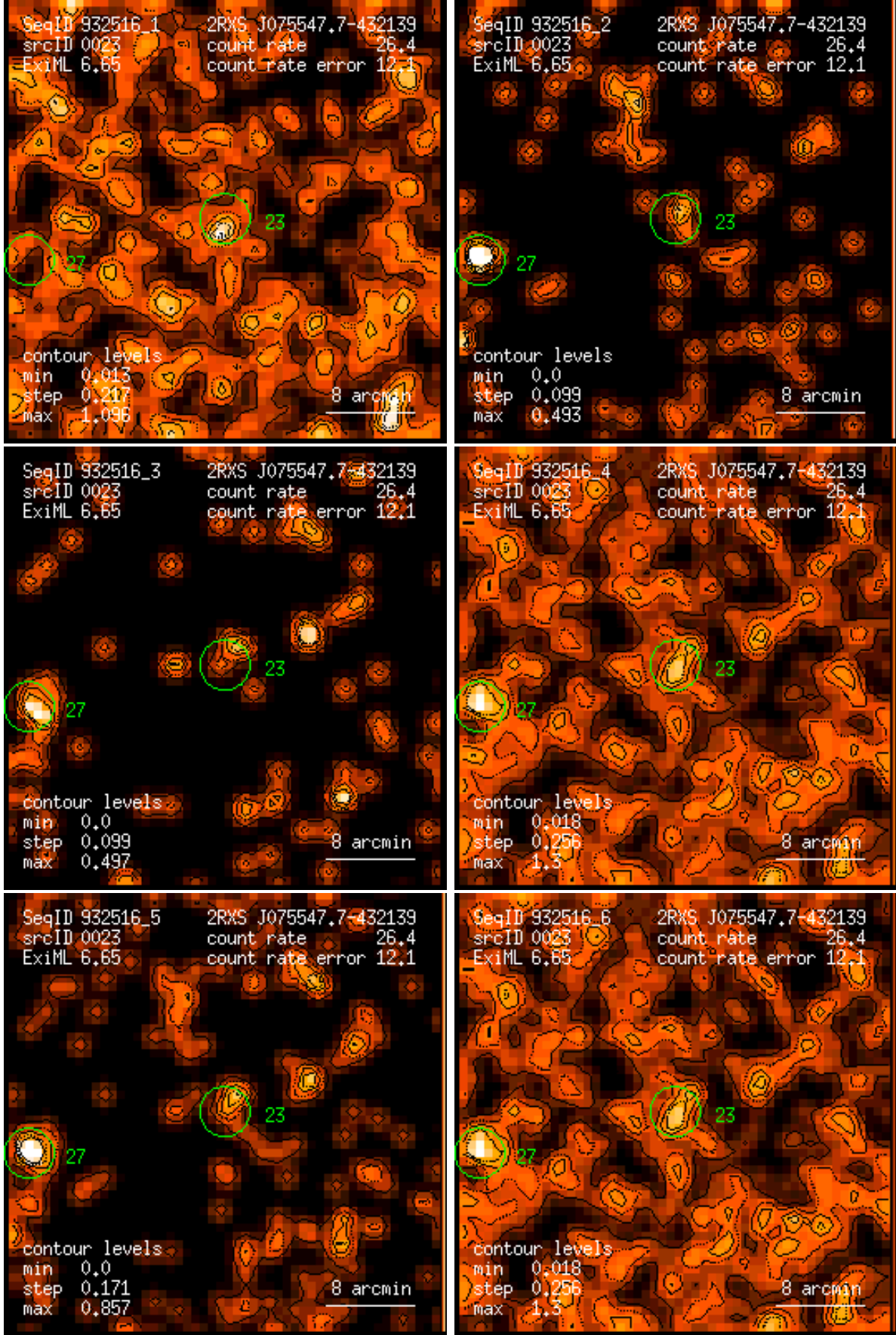
Figure 23: RASS 932516: detection 0023: band rate images, Gaussian filter: (1) PSPC channels 11 – 41, (2) 52 – 90, (3) 91 – 201, (4) 11 – 235, (5) 52 – 201, (6) 11 – 201. Broad band rates in counts/ks. Band rate contour levels in counts/ks/arcmin 2 .
