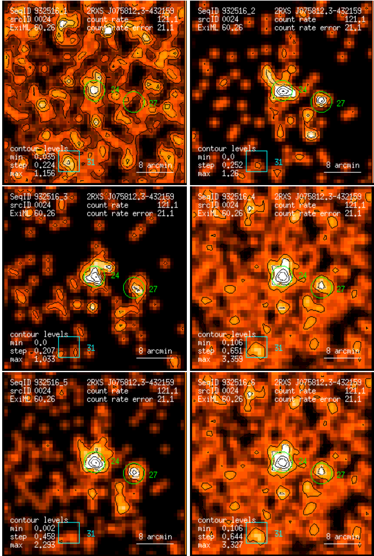
Figure 24: RASS 932516: detection 0024: band rate images, Gaussian filter: (1) PSPC channels 11 – 41, (2) 52 – 90, (3) 91 – 201, (4) 11 – 235, (5) 52 – 201, (6) 11 – 201. Broad band rates in counts/ks. Band rate contour levels in counts/ks/arcmin 2 .
