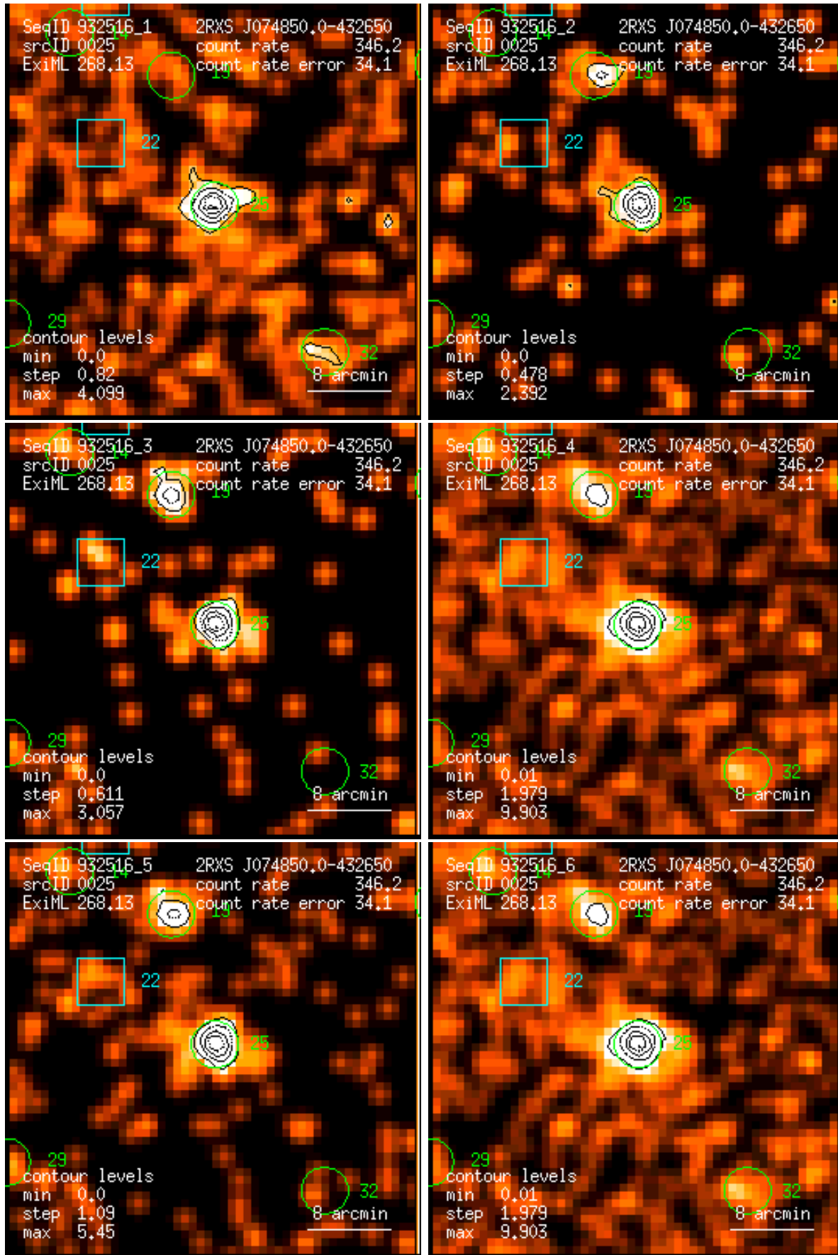
Figure 25: RASS 932516: detection 0025: band rate images, Gaussian filter: (1) PSPC channels 11 – 41, (2) 52 – 90, (3) 91 – 201, (4) 11 – 235, (5) 52 – 201, (6) 11 – 201. Broad band rates in counts/ks. Band rate contour levels in counts/ks/arcmin 2 .
