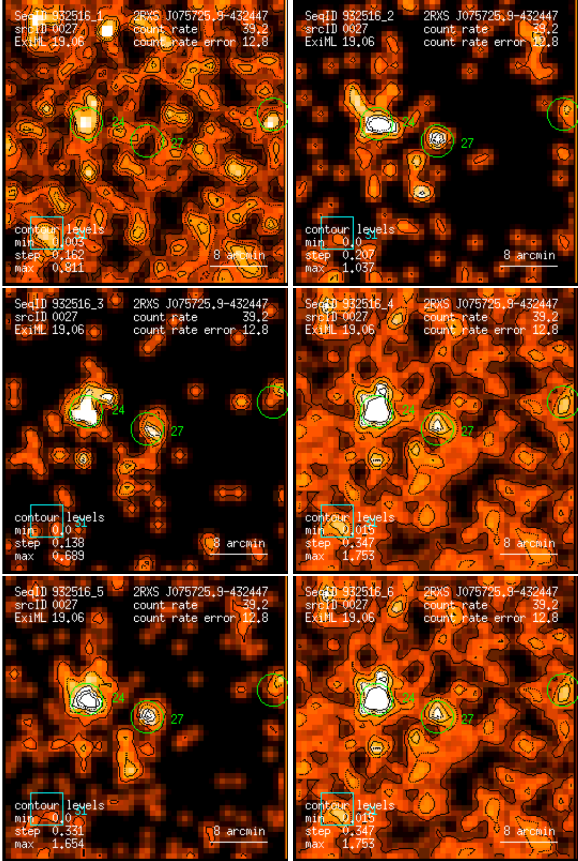
Figure 27: RASS 932516: detection 0027: band rate images, Gaussian filter: (1) PSPC channels 11 – 41, (2) 52 – 90, (3) 91 – 201, (4) 11 – 235, (5) 52 – 201, (6) 11 – 201. Broad band rates in counts/ks. Band rate contour levels in counts/ks/arcmin 2 .
