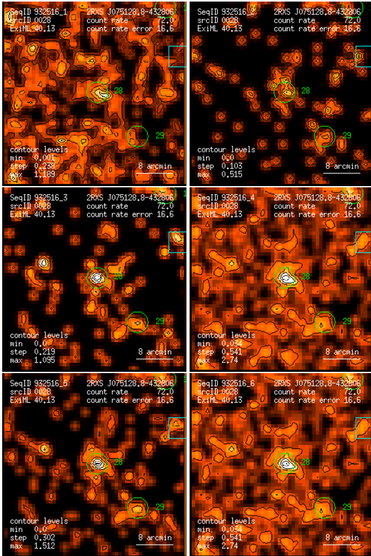
Figure 28: RASS 932516: detection 0028: band rate images, Gaussian filter: (1) PSPC channels 11 – 41, (2) 52 – 90, (3) 91 – 201, (4) 11 – 235, (5) 52 – 201, (6) 11 – 201. Broad band rates in counts/ks. Band rate contour levels in counts/ks/arcmin 2 .
