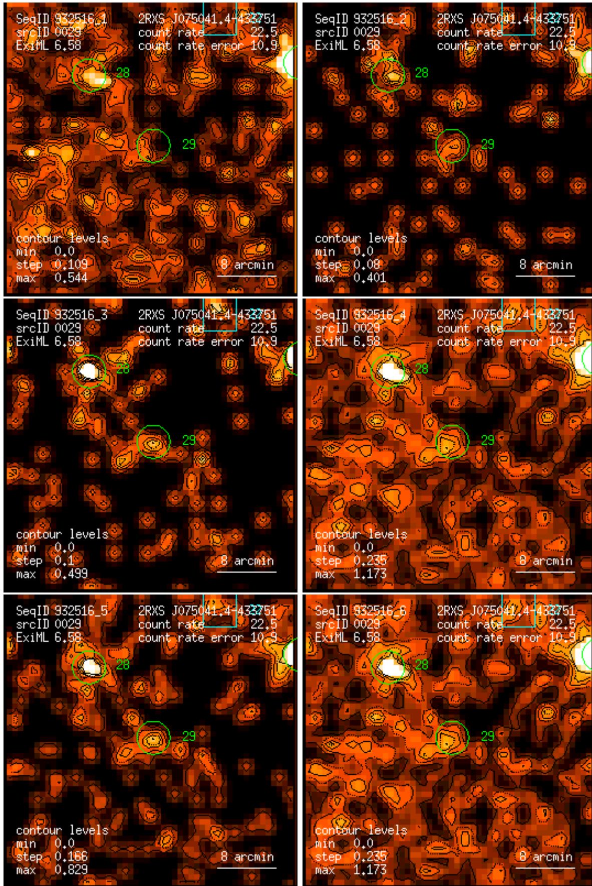
Figure 29: RASS 932516: detection 0029: band rate images, Gaussian filter: (1) PSPC channels 11 – 41, (2) 52 – 90, (3) 91 – 201, (4) 11 – 235, (5) 52 – 201, (6) 11 – 201. Broad band rates in counts/ks. Band rate contour levels in counts/ks/arcmin 2 .
