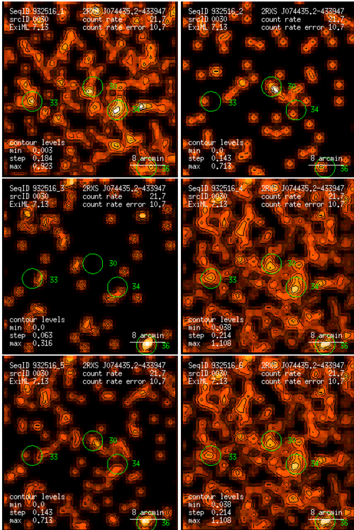
Figure 30: RASS 932516: detection 0030: band rate images, Gaussian filter: (1) PSPC channels 11 – 41, (2) 52 – 90, (3) 91 – 201, (4) 11 – 235, (5) 52 – 201, (6) 11 – 201. Broad band rates in counts/ks. Band rate contour levels in counts/ks/arcmin 2 .
