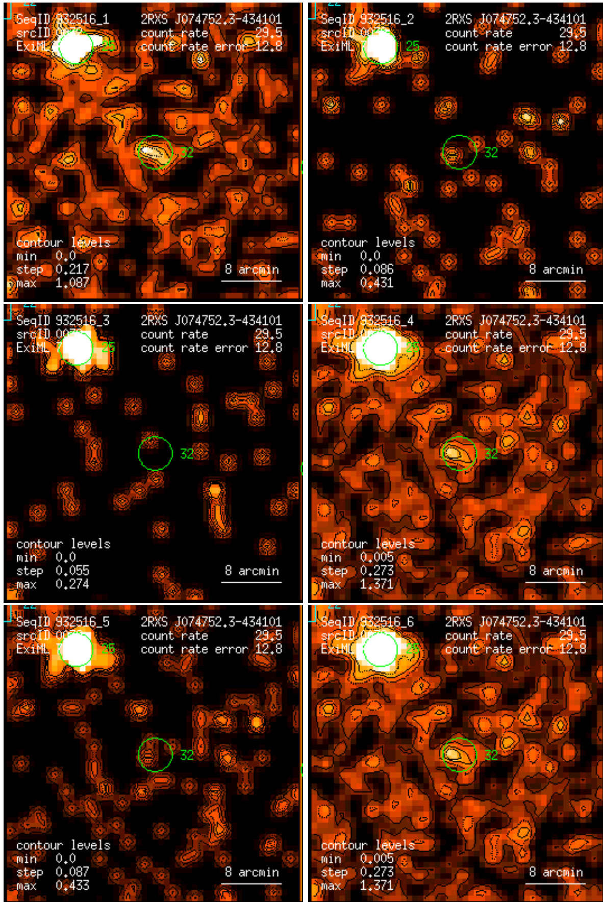
Figure 32: RASS 932516: detection 0032: band rate images, Gaussian filter: (1) PSPC channels 11 – 41, (2) 52 – 90, (3) 91 – 201, (4) 11 – 235, (5) 52 – 201, (6) 11 – 201. Broad band rates in counts/ks. Band rate contour levels in counts/ks/arcmin 2 .
