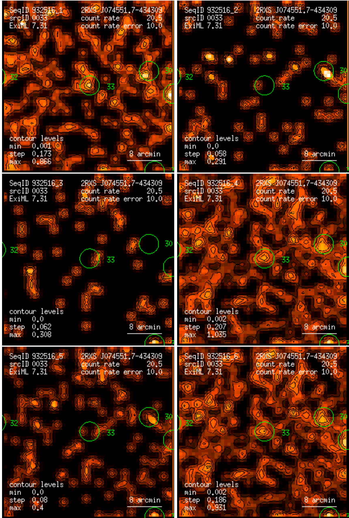
Figure 33: RASS 932516: detection 0033: band rate images, Gaussian filter: (1) PSPC channels 11 – 41, (2) 52 – 90, (3) 91 – 201, (4) 11 – 235, (5) 52 – 201, (6) 11 – 201. Broad band rates in counts/ks. Band rate contour levels in counts/ks/arcmin 2 .
