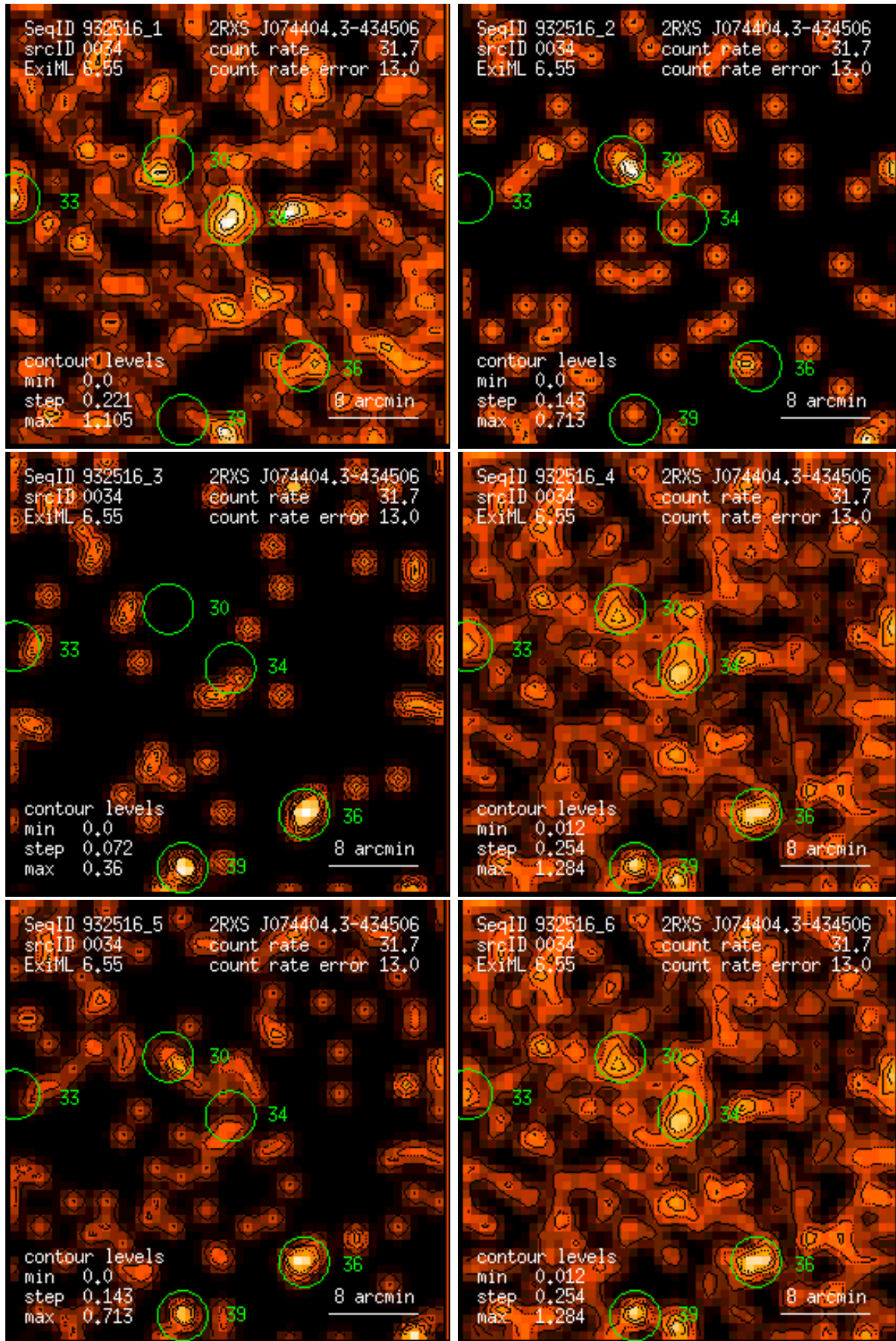
Figure 34: RASS 932516: detection 0034: band rate images, Gaussian filter: (1) PSPC channels 11 – 41, (2) 52 – 90, (3) 91 – 201, (4) 11 – 235, (5) 52 – 201, (6) 11 – 201. Broad band rates in counts/ks. Band rate contour levels in counts/ks/arcmin 2 .
