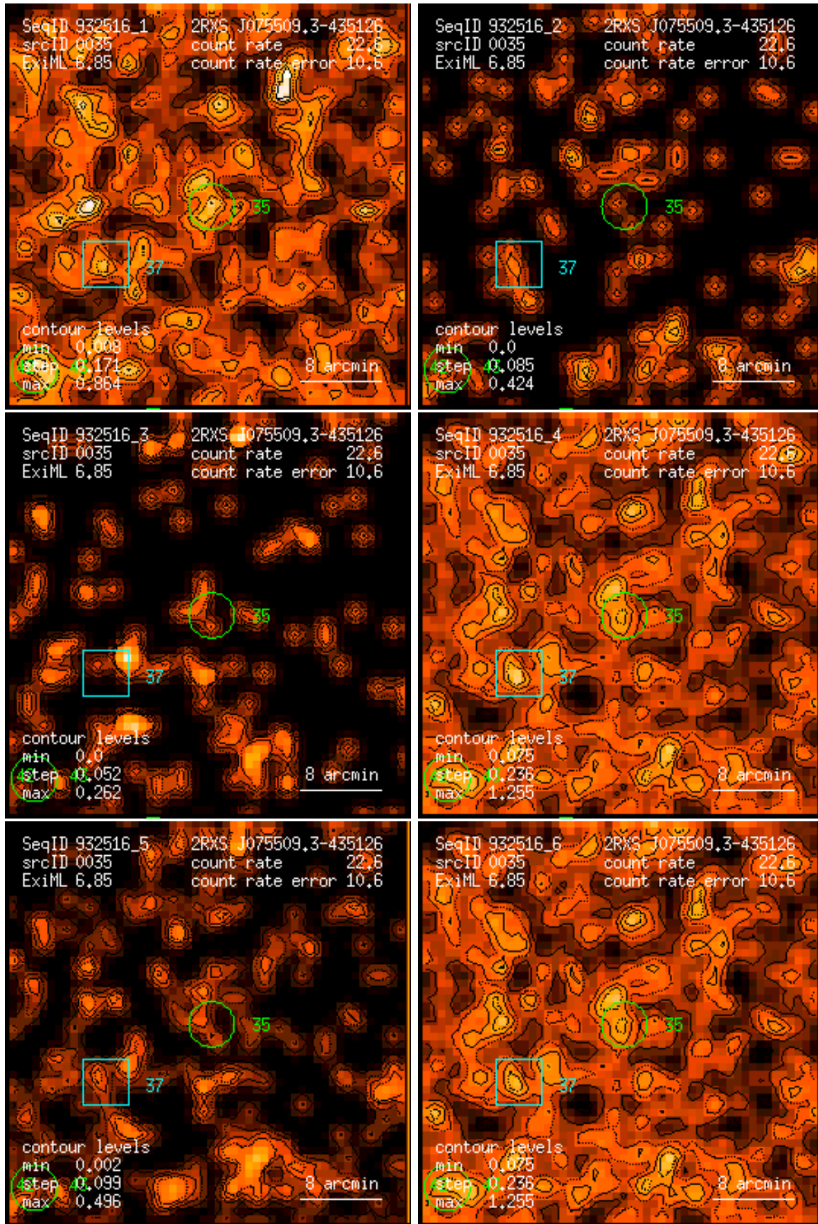
Figure 35: RASS 932516: detection 0035: band rate images, Gaussian filter: (1) PSPC channels 11 – 41, (2) 52 – 90, (3) 91 – 201, (4) 11 – 235, (5) 52 – 201, (6) 11 – 201. Broad band rates in counts/ks. Band rate contour levels in counts/ks/arcmin 2 .
