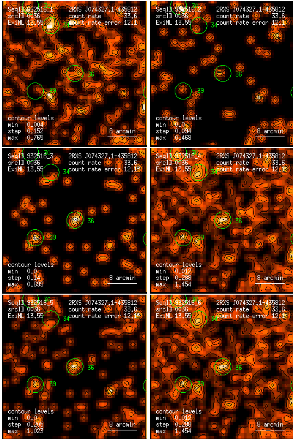
Figure 36: RASS 932516: detection 0036: band rate images, Gaussian filter: (1) PSPC channels 11 – 41, (2) 52 – 90, (3) 91 – 201, (4) 11 – 235, (5) 52 – 201, (6) 11 – 201. Broad band rates in counts/ks. Band rate contour levels in counts/ks/arcmin 2 .
