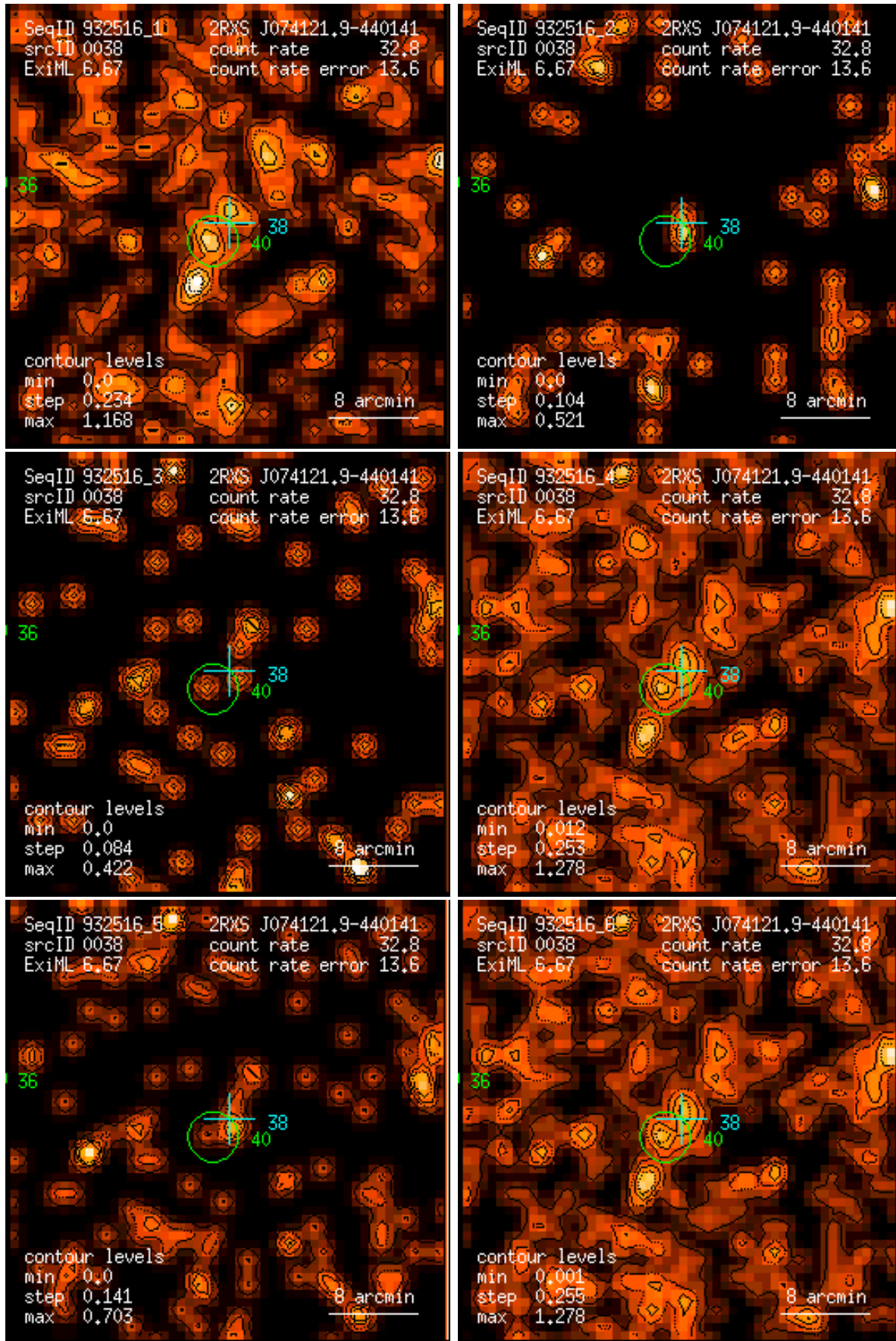
Figure 38: RASS 932516: detection 0038: band rate images, Gaussian filter: (1) PSPC channels 11 – 41, (2) 52 – 90, (3) 91 – 201, (4) 11 – 235, (5) 52 – 201, (6) 11 – 201. Broad band rates in counts/ks. Band rate contour levels in counts/ks/arcmin 2 .
