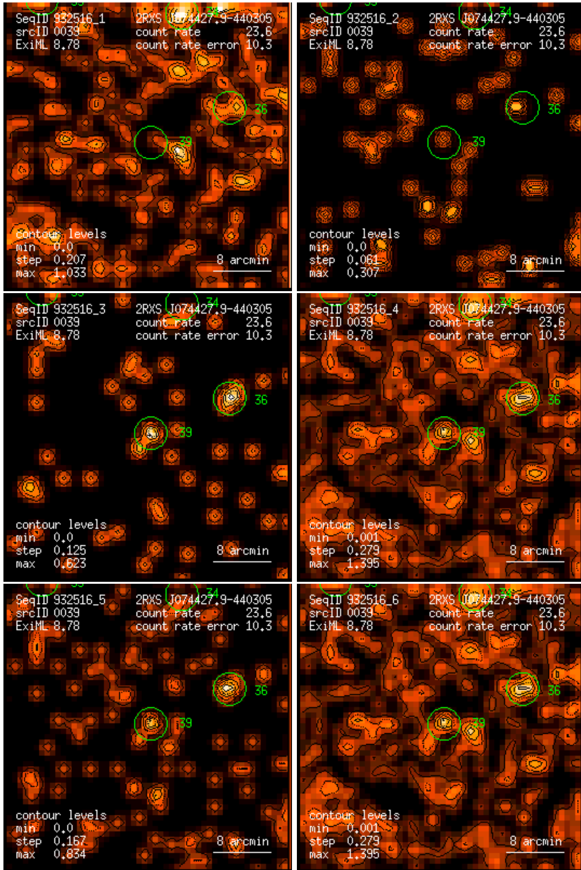
Figure 39: RASS 932516: detection 0039: band rate images, Gaussian filter: (1) PSPC channels 11 – 41, (2) 52 – 90, (3) 91 – 201, (4) 11 – 235, (5) 52 – 201, (6) 11 – 201. Broad band rates in counts/ks. Band rate contour levels in counts/ks/arcmin 2 .
