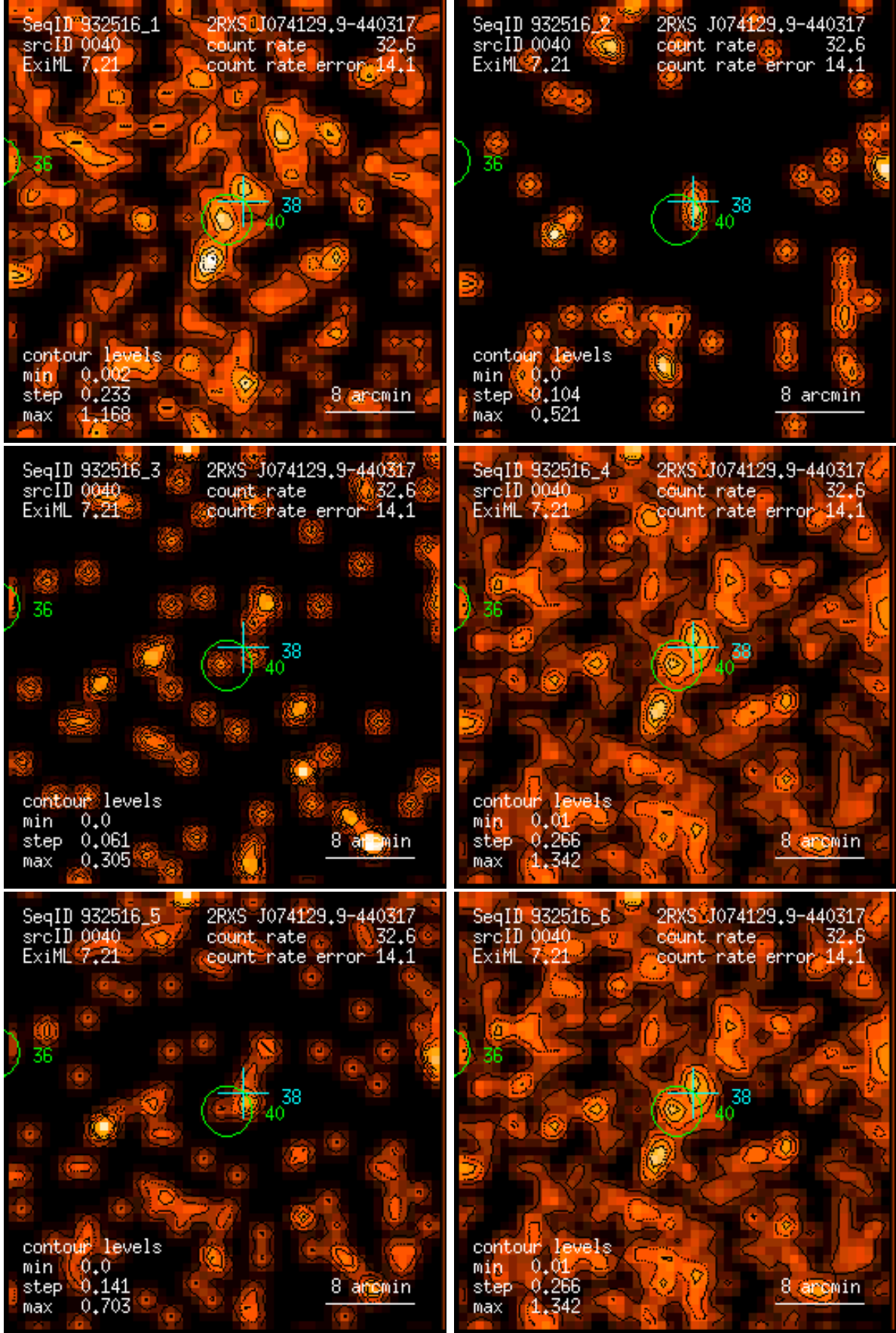
Figure 40: RASS 932516: detection 0040: band rate images, Gaussian filter: (1) PSPC channels 11 – 41, (2) 52 – 90, (3) 91 – 201, (4) 11 – 235, (5) 52 – 201, (6) 11 – 201. Broad band rates in counts/ks. Band rate contour levels in counts/ks/arcmin 2 .
