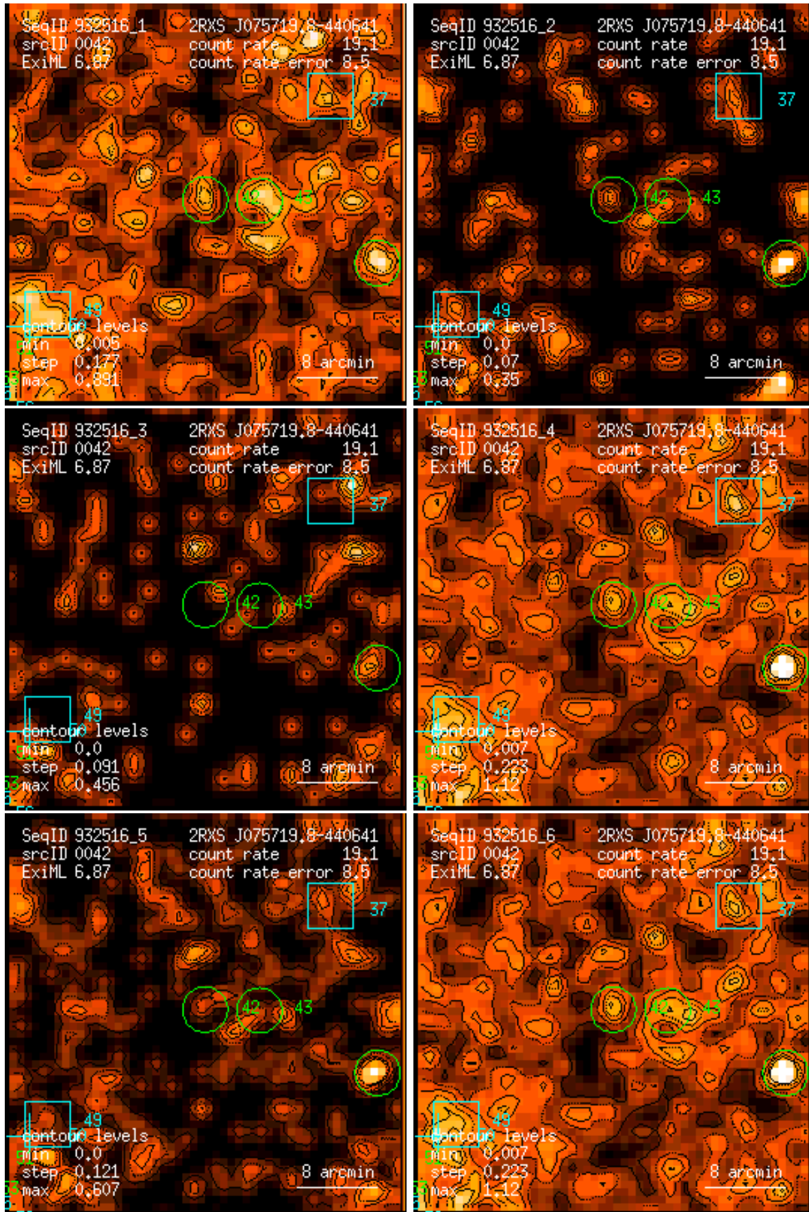
Figure 42: RASS 932516: detection 0042: band rate images, Gaussian filter: (1) PSPC channels 11 – 41, (2) 52 – 90, (3) 91 – 201, (4) 11 – 235, (5) 52 – 201, (6) 11 – 201. Broad band rates in counts/ks. Band rate contour levels in counts/ks/arcmin 2 .
